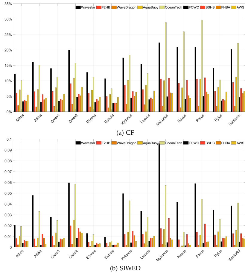
Fig. 5. Greece points estimation of for all WECs.
