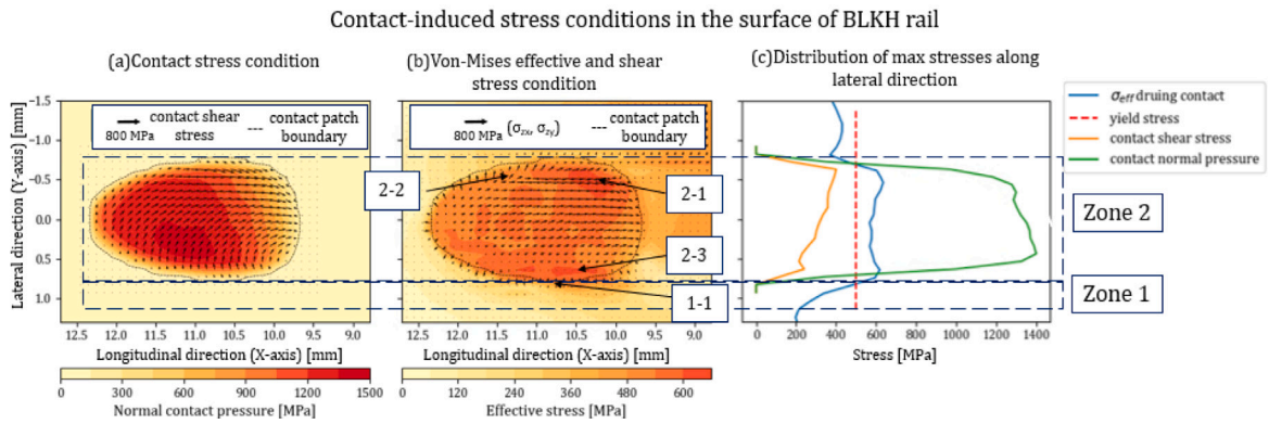
Fig. 14. Contract-induced stress conditions in Zones 1 and 2: (a) surface contact stress conditions simulated with the BLKH rail, (b) effective stress conditions in the surface elements during contact, and (c) distribution of maximum normal contact pressure, shear stress and effective stress in surface elements.
