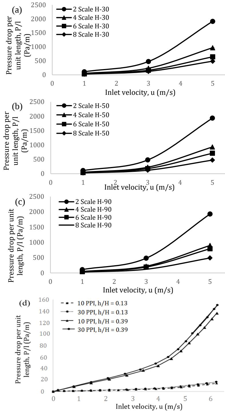
Figure 10: Pressure drops of 3D printed foam at different measuring heightst; (a) 0.03m, (b) 0.05m, and (c) 0.09m and (d) 10 PPI and 30 PPI (Shikh Anuar, et al., 2018b).
