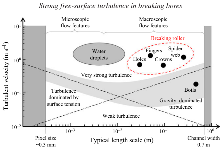
Figure 4. Typical length and velocity scales of main turbulent air–water surface features observed in breaking bores. Present data are plotted against the length–velocity graph by Brocchini & Peregrine (2001a).
