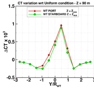
a - Thrust coefficient
