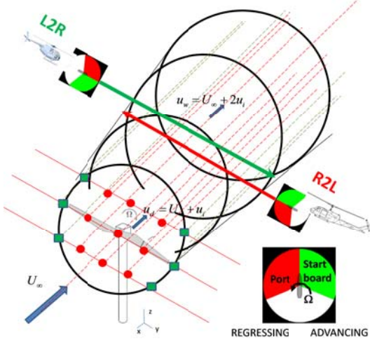
Figure 1: Description of the helicopter approaching the WT wake
