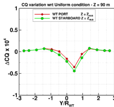
b - Torque coefficient
