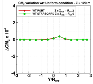
Figure 22: Variation of the helicopter moment coefficients with respect to the uniform conditions at the heights 60 m, 90 m, 120 m, respectively. Helicopter leaving the WT disk on its port side R2L (red) or starboard side L2R (green) while crossing the WT wake
