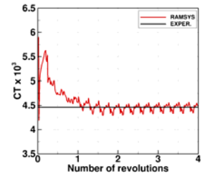
Figure 10: Thrust coefficient time history
