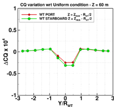
Figure 23: Variation of the rotor thrust coefficient (top) and bottom coefficient (bottom) with respect to the uniform conditions at the heights 60 m, 90 m, 120 m respectively. Helicopter leaving the WT disk on its port side R2L (red) or starboard side L2R (green) while crossing the WT wake
