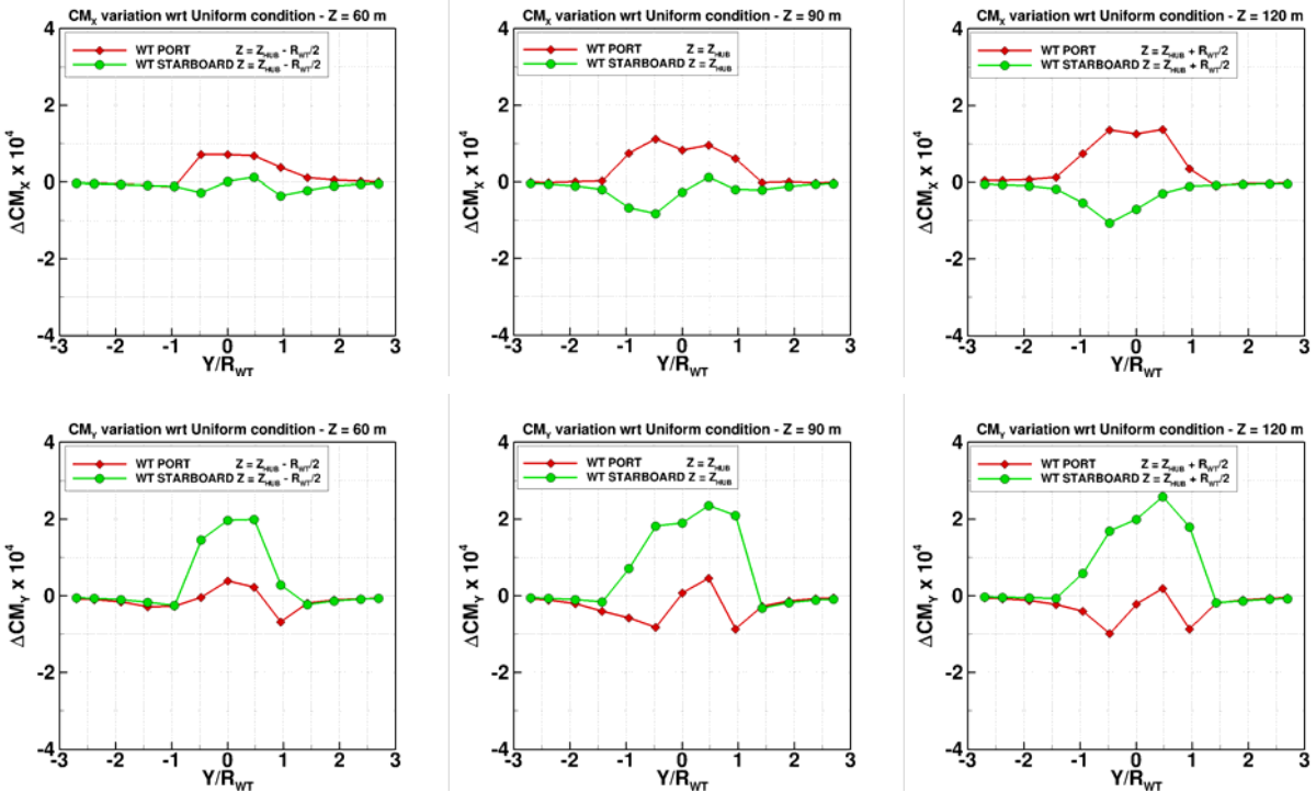
a - Rolling moment coefficient
