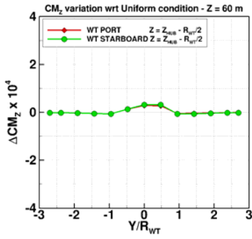
Figure 22: Variation of the helicopter moment coefficients with respect to the uniform conditions at the heights 60 m, 90 m, 120 m, respectively. Helicopter leaving the WT disk on its port side R2L (red) or starboard side L2R (green) while crossing the WT wake
