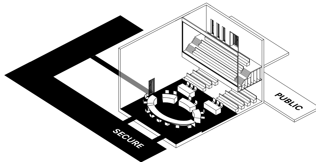
courtroom module with grandstand
