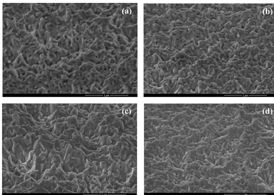
Fig. 7. SEM images of the 4 outer boundaries of the textured layers. (a) 100 °C and 1.5 μbar (b) 100 °C and 3.5 μbar (c) 150 °C and 1.5 μbar (d) 150 °C and 3.5 μbar.
