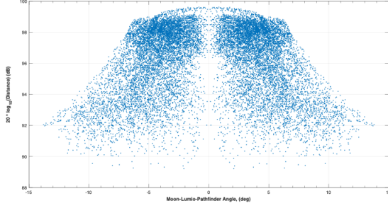
Fig. 11: Lunar Pathfinder viewing angles (with respect to the Moon Center) during the operational phase
