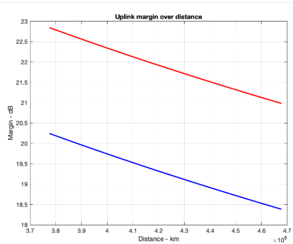
Fig. 9: DTE uplink margin
