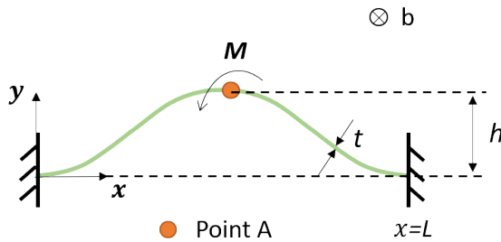
Figure D.1: Model a curved beam under a moment applied in the middle. The geometry of the beam-unit is described based on the depicted x - y coordinate system. A moment is applied at Point A ( x = L/2 ).
