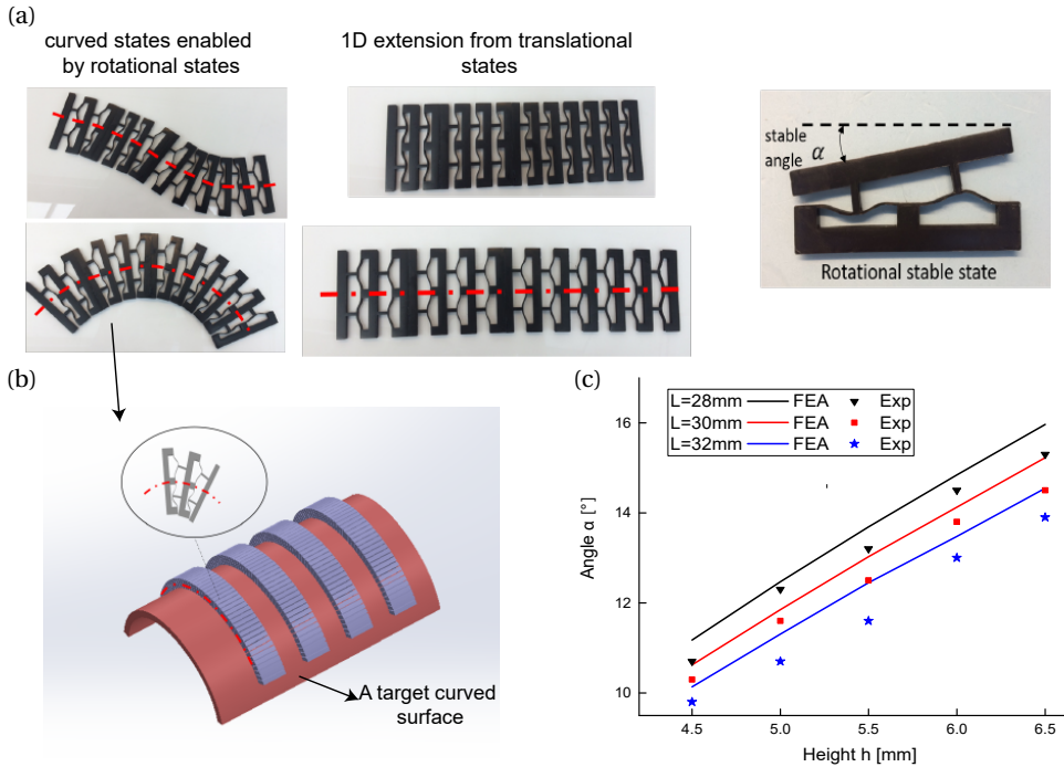
Figure 2.9: Demonstrations of conformal-morphing on a curved surface based on the rotational stable states. (a) An ensemble of unit cells stacked in series. By deforming in different transition modes, it can switch to curved shapes with different curvatures. The angle \alpha is the stable angle achieved by a single unit's rotational transitions. (b) An illustrative example of conformal morphing on a spatial free-form surface. To realize shape-matching, our deformed metastructures (grey) can deform into a curved shape to match the target curved free-form shape (red). (c) The stable angle ( \alpha ) is characterized experimentally and numerically, as a function of h for different L .
