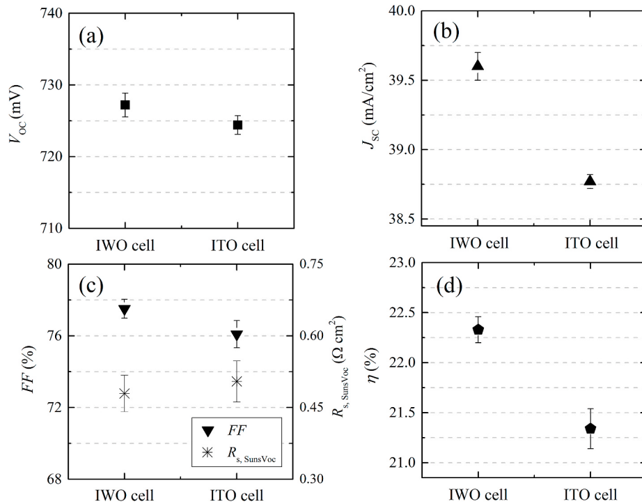
Fig. 7. (a) Open-circuit voltage, V_{OC} , (b) short-circuit current density, J_{SC} , (c) fill factor, FF , and series resistance, R_s , R_{s, \text{SunsVoc}} , and (d) illuminated area power conversion efficiency, \eta of the IWO- and ITO-based SHJ devices. The cell area is 8.97 \text{ cm}^2 and the metal coverage is 1.93%. The results are based on five batches of cells.
