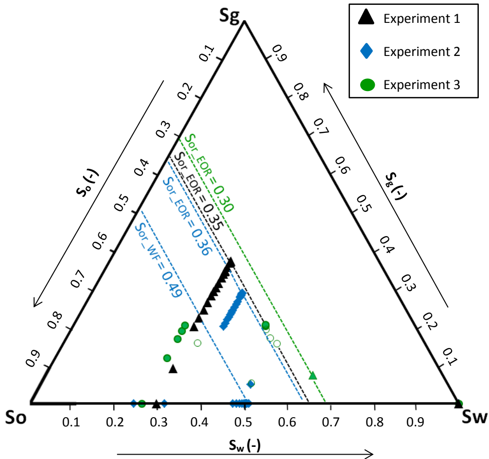
Figure 12: Saturation paths for Exp. 1, Exp. 2 and Exp. 3. S_{wr} , S_{or} , S_{gr} , S_{or\_WF} and S_{or\_EOR} represent the water, oil, gas, residual oil to waterflood and residual oil to immiscible gas/WAG respectively. Three-phase saturations shown were averaged over the entire core and calculated using material balance calculations. The closed and open circles in Exp. 3 represent the gas and water injection during the first two WAG cycles respectively. The green triangle indicates the saturation distribution after successfully injecting 12 full WAG cycles.
