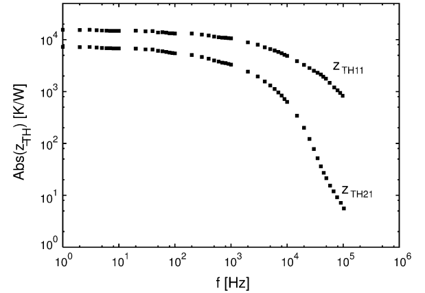
Fig. 5. Extracted magnitude of \tilde{z}_{TH11} and \tilde{z}_{TH21} for the test structure T-6.
