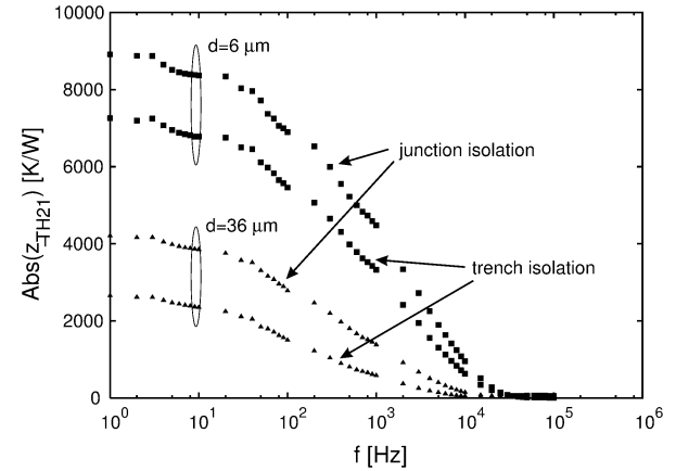
Fig. 7. Comparison between magnitudes of the mutual thermal coupling impedance \underline{z}_{TH21} for the trench and junction isolated test structures.
