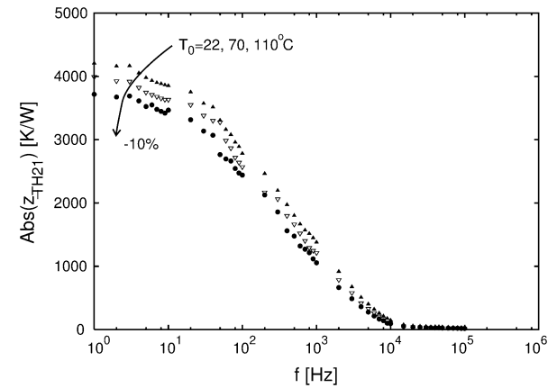
Fig. 8. Temperature dependence of the extracted magnitude of \underline{z}_{TH21} for the test structure J-36.
