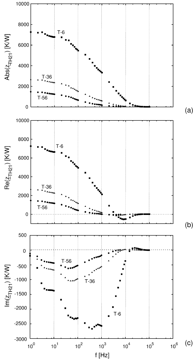
Fig. 6. Extracted (a) magnitude, (b) real and (c) imaginary part of \underline{z}_{TH21} for the test structures T-6, T-36, and T-56.
