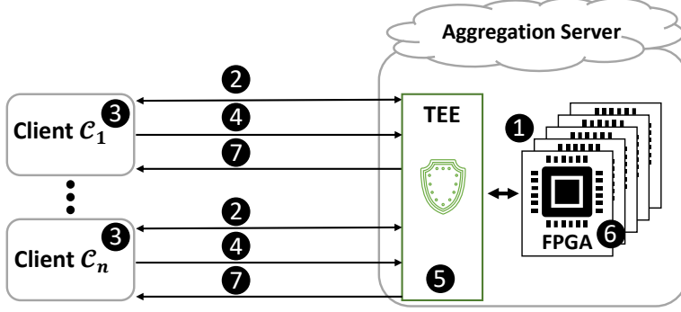
Figure 5.1: Workflow of FLAIRS.
