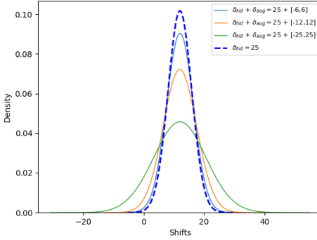
(a) Trace desynchronization distribution for different values of \delta_{aug} when measurements contain desynchronization of \delta_{hid} = 25 .
