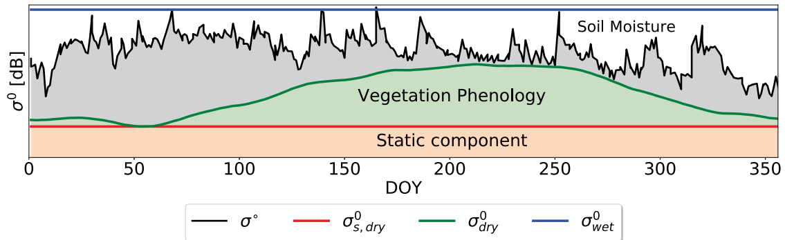
Fig. 1. Illustration of the wet reference ( \sigma_{\text{wet}}^0 ), and static components ( \sigma_{\text{s,dry}}^0 ) and dynamic components of the dry reference ( \sigma_{\text{dry}}^0 ) as three components of the TU Wien soil moisture retrieval method along with radar backscatter coefficient (Steele-Dunne et al., 2019). (For interpretation of the references to color in this figure legend, the reader is referred to the web version of this article.)
