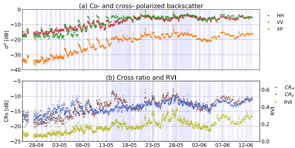
Fig. 6. Complete time series of L-band (a) HH, VV, and cross-polarized (XP) radar backscatter, and (b) CRs ( CR_V , and CR_H ) and Radar Vegetation Index (RVI). Light blue vertical lines indicate the presence of SCW during the radar acquisition. (For interpretation of the references to color in this figure legend, the reader is referred to the web version of this article.)
