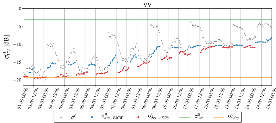
Fig. 10. Time series of radar backscatter along with the calculated static component ( \sigma_{s,dry}^0 ), the dry reference for wet vegetation ( \sigma_{dry-PSCW}^0 ) and dry vegetation ( \sigma_{dry-ASCW}^0 ), and the wet reference ( \sigma_{wet}^0 ) for VV-pol and period of 3 to 15 May. (For interpretation of the references to color in this figure legend, the reader is referred to the web version of this article.)
