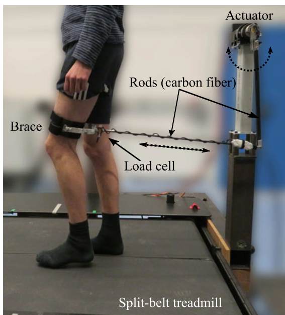
Fig. 1 Overview of the LOPER (Lower limb PERTurbator). The rotary actuator is placed on a steel support frame. The rotational actuator motion is converted to a linear motion through the carbon-fiber rods with a ball joint linkage. The motion is transferred into the human leg through an aluminum frame with brace connected to the user. The load cell measuring interaction forces is placed between the aluminum frame and carbon-fiber rod
