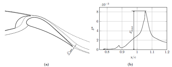
Fig. 6: Maximum displacement thickness max of the flap wake.
