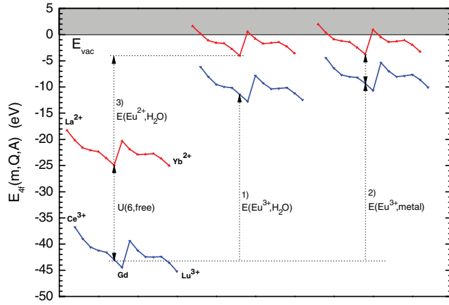
FIG. 5. (Color online) Scheme with the 4f-VRBE E_{4f}(m, Q, A) of the divalent ( Q = 2+ ; upper curves) and trivalent ( Q = 3+ ; lower curves) lanthanide ions. The curves on the left pertain to A = \text{vacuum} , in the middle to A = \text{H}_2\text{O} , and on the right to A = \text{metal} . The size of the chemical shift E(\text{Eu}^Q, A) and the Coulomb repulsion energy U(6, A) for Eu are indicated by the arrows.
