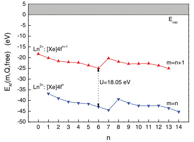
FIG. 2. (Color online) 4f-VRBE curves for the free trivalent lanthanide ions (lower curve) and free divalent (upper curve) lanthanide ions.
