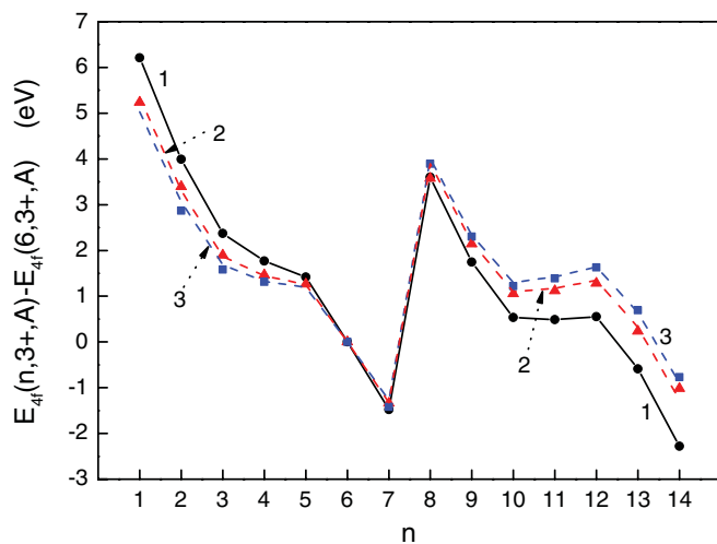
FIG. 6. (Color online) 4f-electron binding energies relative to that in \text{Eu}^{3+} . • and solid curve 1 is for the free trivalent lanthanide ions, dashed curve 2 is obtained with a contraction tilt \alpha(3+, A) = 0.11 \text{ eV/pm} on curve 1, dashed curve 3 is obtained with a contraction tilt \alpha(3+, A) = 0.15 \text{ eV/pm} on curve 1. ■ data symbols pertain to the lanthanide metals. ▲ data symbols pertain to \text{YPO}_4 .
