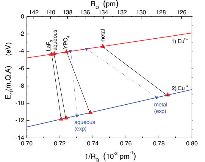
FIG. 10. (Color online) Lines 1 and 2 are the 4f-VRBE lines for \text{Eu}^{2+} and \text{Eu}^{3+} as defined within the screening model. ▲, 4f-VRBE data for Eu calculated by using Eq. (10) and U(6, A) = 7.51, 7.42, 7.0 , and 5.61 eV for \text{LaF}_3 , aqueous solution, \text{YPO}_4 , and Eu metal. ▼ are experimental 4f-VRBE values for aqueous solutions and Eu metal.
