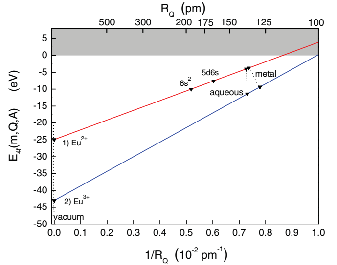
FIG. 8. (Color online) The 4f-VRBE as function of the inverse screening distance for line 1 \text{Eu}^{2+} with [\text{Xe}]4f^7 configuration and line 2 \text{Eu}^{3+} with [\text{Xe}]4f^6 configuration. ▼ data symbols are experimentally derived binding energies.
