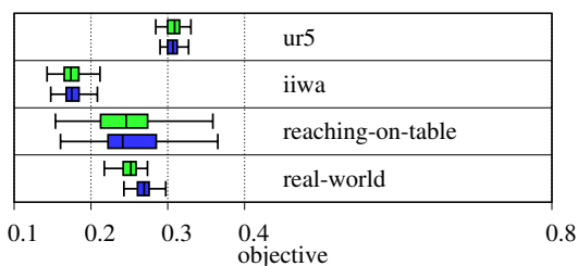
Fig. 6: The autotuned for the panda robot in simulation for the reaching-in-ring scenario on modified scenarios (blue) is compared to autotuned parameter sets obtained on these scenarios directly (green). Exchanging the robot (ur5, iiwa) and changing the scenario ( reaching-on-table ) results in a very small loss in performance, while the loss is higher when parameters are transferred between simulation and real world (real-world).
