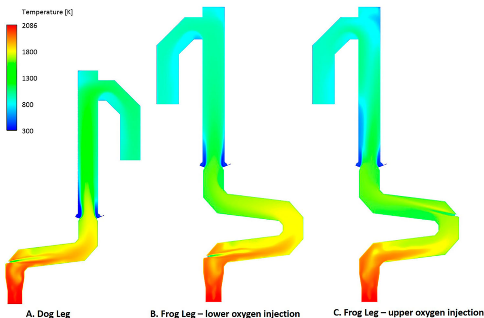
Figure 8. Temperature contours for different off-gas designs.
