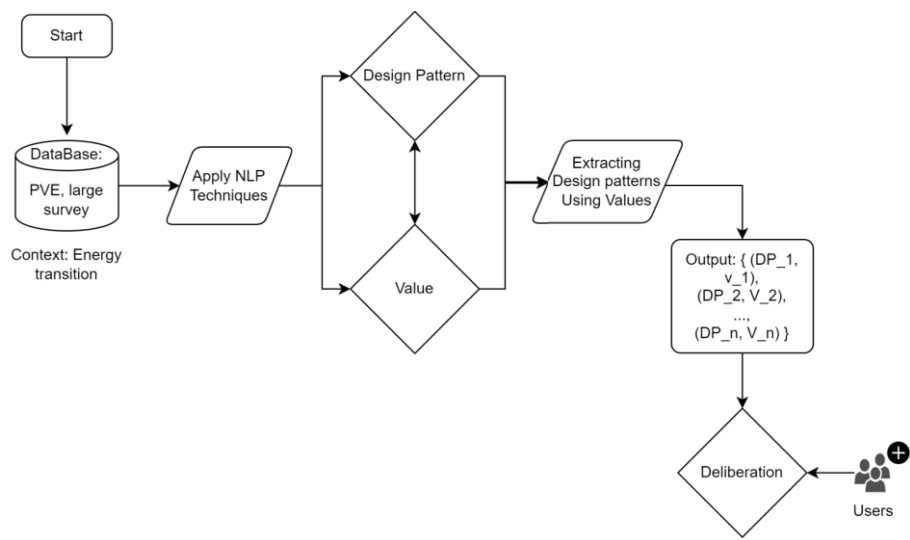
Figure 1. The flowchart illustrates how all three concepts (Design pattern, Value, Deliberation) are related
