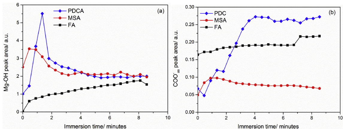
Fig. 11. In situ ATR-FTIR results (a) Mg-OH peak and (b) asymmetric carboxylate peak area evolution during immersion in PDC, MSA and FA solution.
