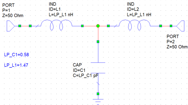
FIGURE 5. LC circuit representation of the low-pass filtering phenomenon at dipole edges.
