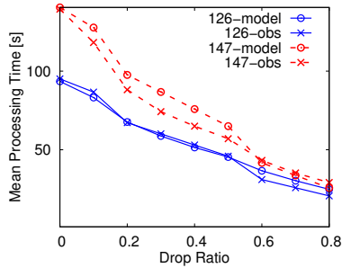
Figure 4. Job processing times and drop ratio.
