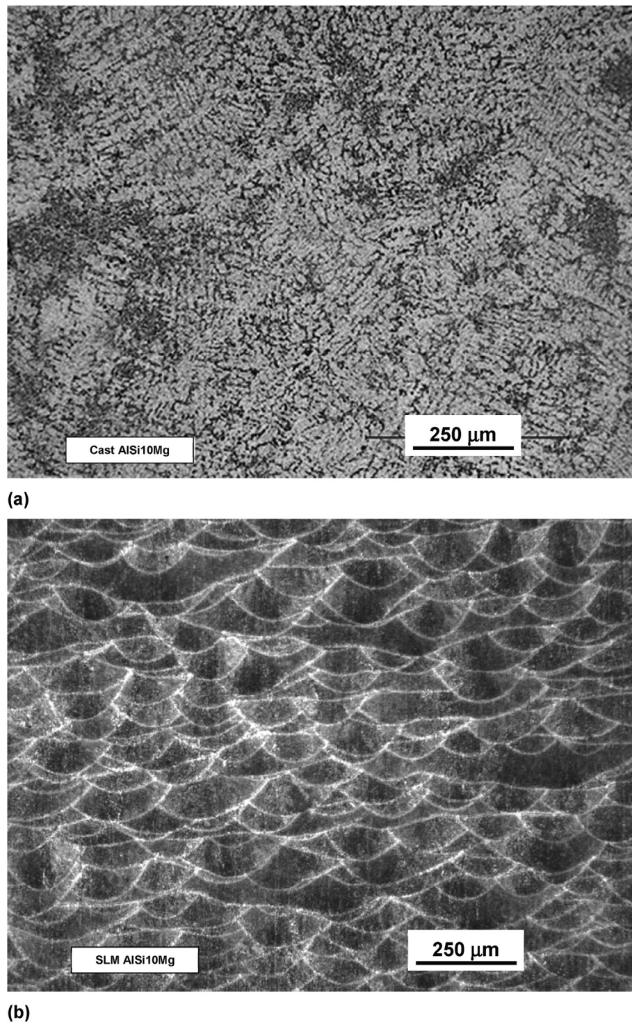
Fig. 1. Optical micrographs of (a) as-cast, (b) as-printed AlSi10Mg.
