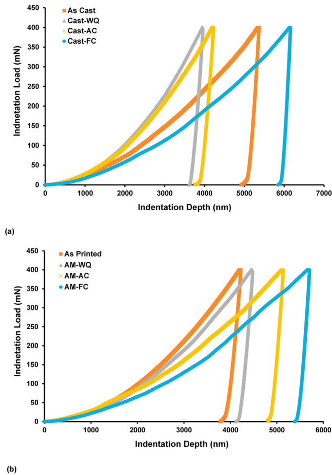
Fig. 12. Representative load-depth curves (a) cast, (b) SLM AlSi10Mg.
