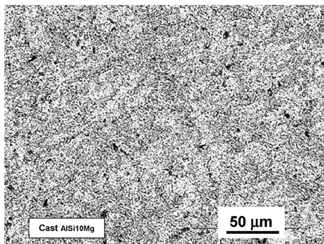
Fig. 3. Optical micrographs of various heat-treated cast AlSi10Mg, (a) water quenched (WQ); (b) air cooled (AC); (c) furnace cooled (FC).
