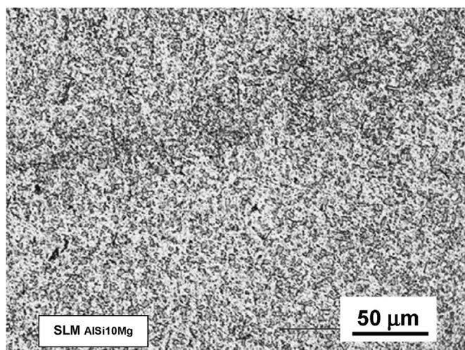
Fig. 4. Optical micrographs of various heat-treated SLM AlSi10Mg, (a) water quenched (WQ); (b) air cooled (AC); (c) furnace cooled (FC).
