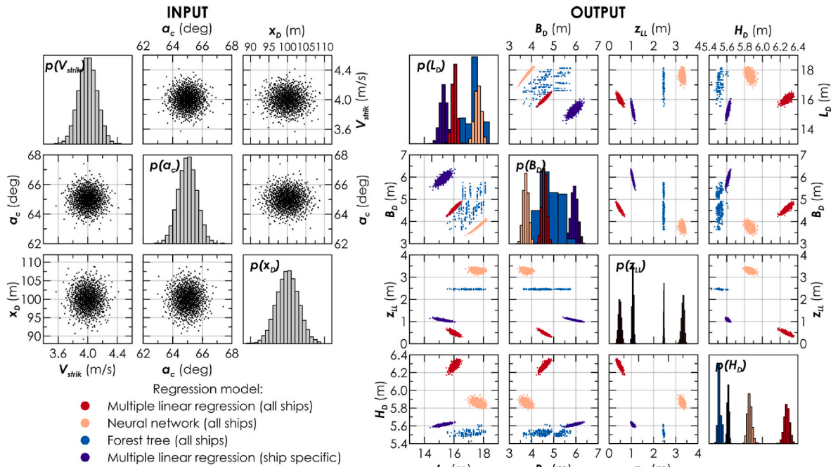
Fig. 13. Breach dimensions prediction according to different regression models for V_{strik} = 4.0 m/s.
