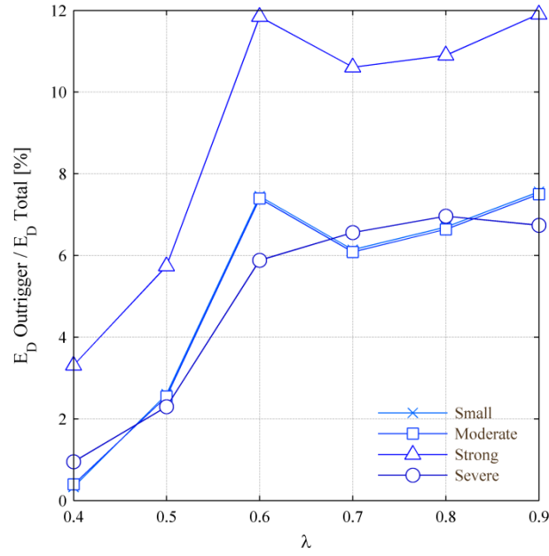
Figure 23: Damping energy (in %) dissipated only by the outriggers, under the combined influence of \lambda and different earthquake levels of 1940 El Centro earthquake; C_d = 1.18E+05 \text{ kN-s/m} and \zeta = 2.0\% .
