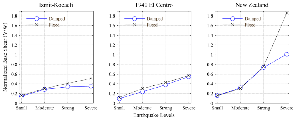
Figure 30: Normalized base shear ( V ) over seismic mass ( W ) of the fixed and damped outrigger under different earthquake levels. \lambda=0.7 , \zeta=2.0\% and C_d=1.18E+05\text{kN}\cdot\text{s/m} (damped outrigger).
