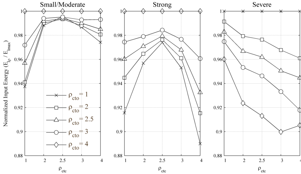
Figure 20: Variations of the Normalized Input Energy ( E_{Ip}/E_{Imax} ), according to combined effect of \rho_{cto} and \rho_{ctc} , under different earthquake levels of 1940 El Centro earthquake; C_d = 1.18E+05kN-s/m , \lambda=0.7 and \zeta=1.5\% .
