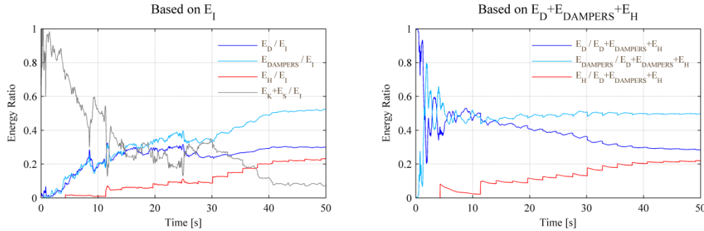
Figure 21: Energy ratios based on E_I and E_D+E_{dampers}+E_H , for the damped outrigger under strong earthquake level of 1940 El Centro earthquake; C_d=1.18E+05\text{kN-s/m} , \lambda=0.7 and \zeta=2.0\% .
