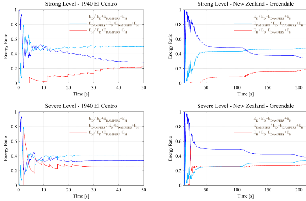
Figure 22: Energy Ratios of the damped outrigger ( C_d = 1.18E+05 \text{ kN-s/m} , \lambda = 0.7 and \zeta = 2.0\% ), under strong and severe levels of 1940 El Centro and New Zealand – Greendale earthquakes
