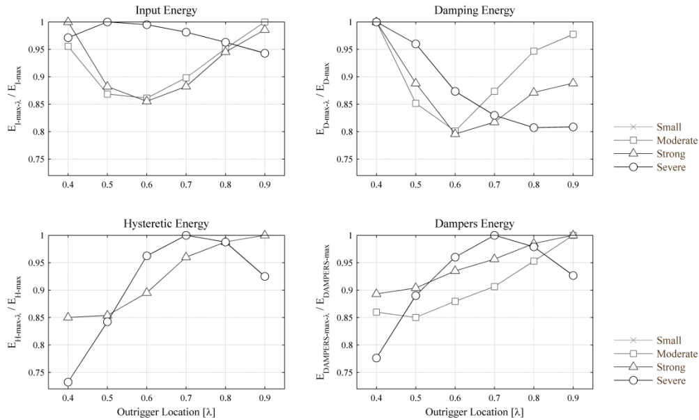
Figure 12: Normalized (actual/maximum) energy distributions of the outrigger structure ( \zeta=2\% - C_d=1.18E+05\text{kN}\cdot\text{s/m} ) according to outrigger location ( \lambda=0.4 - 0.9 ) under four intensity levels of 1940 El Centro earthquake.
