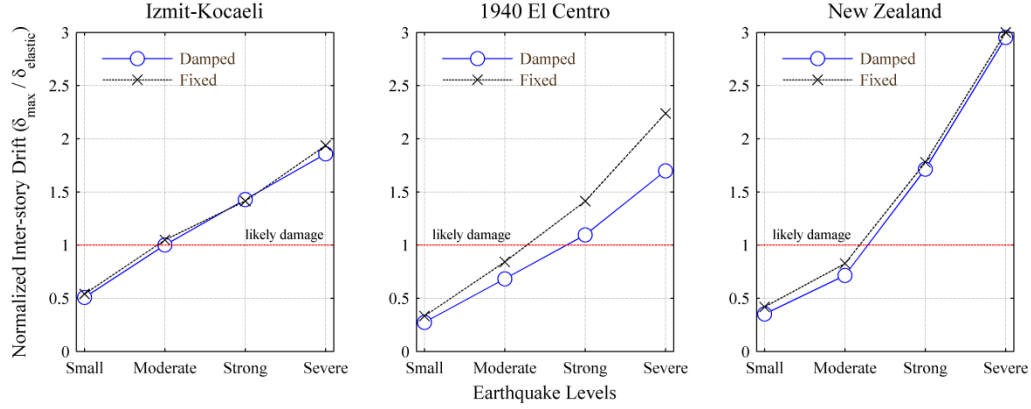
Figure 29: Normalized inter-story drift (maximum/elastic) of the fixed and damped outriggers under different earthquake levels. \lambda=0.7 , \zeta=2.0\% and C_d=1.18E+05\text{kN}\cdot\text{s/m} (damped outrigger).
