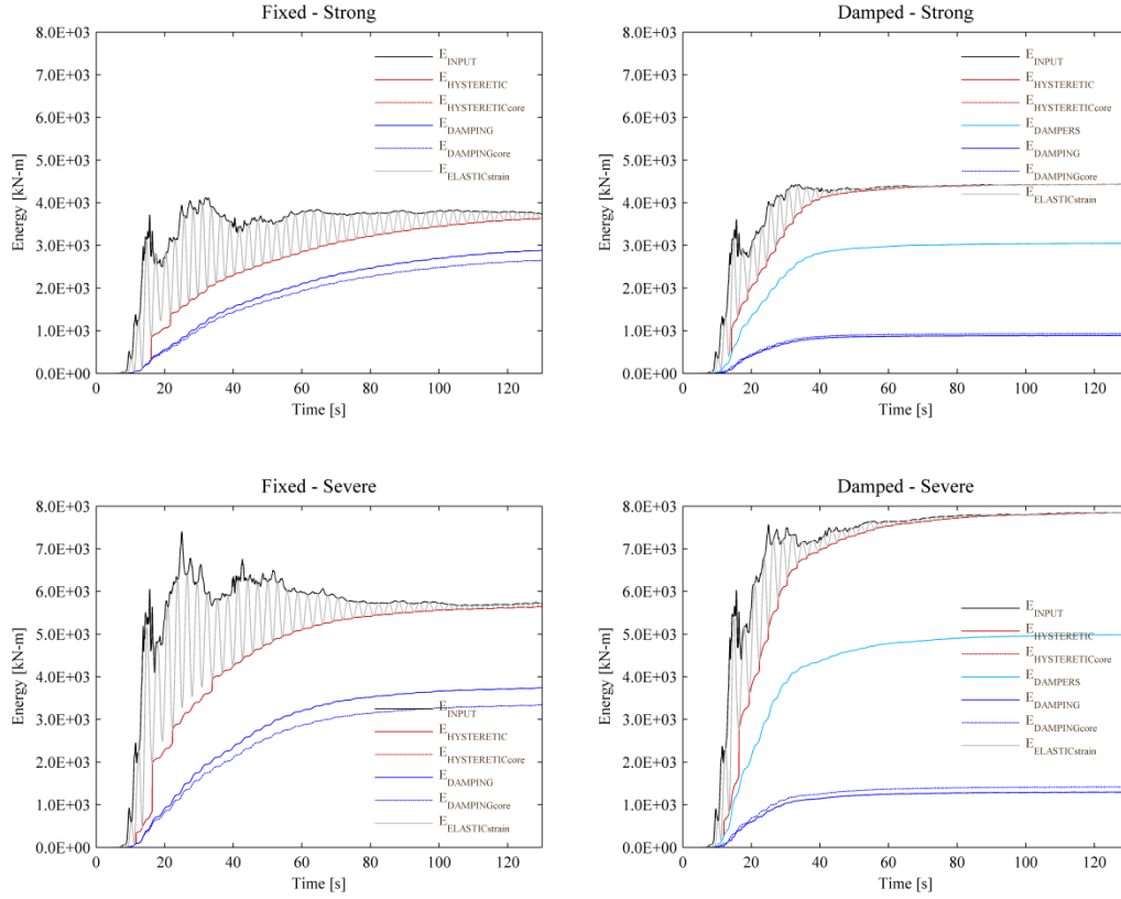
Figure 26: Energy distribution of the fixed and 1.18E+05 \text{ kN-s/m} damped outrigger structures under strong and severe levels of Izmit-Kocaeli earthquake ( \lambda=0.7 and \zeta=2.0\% ).
