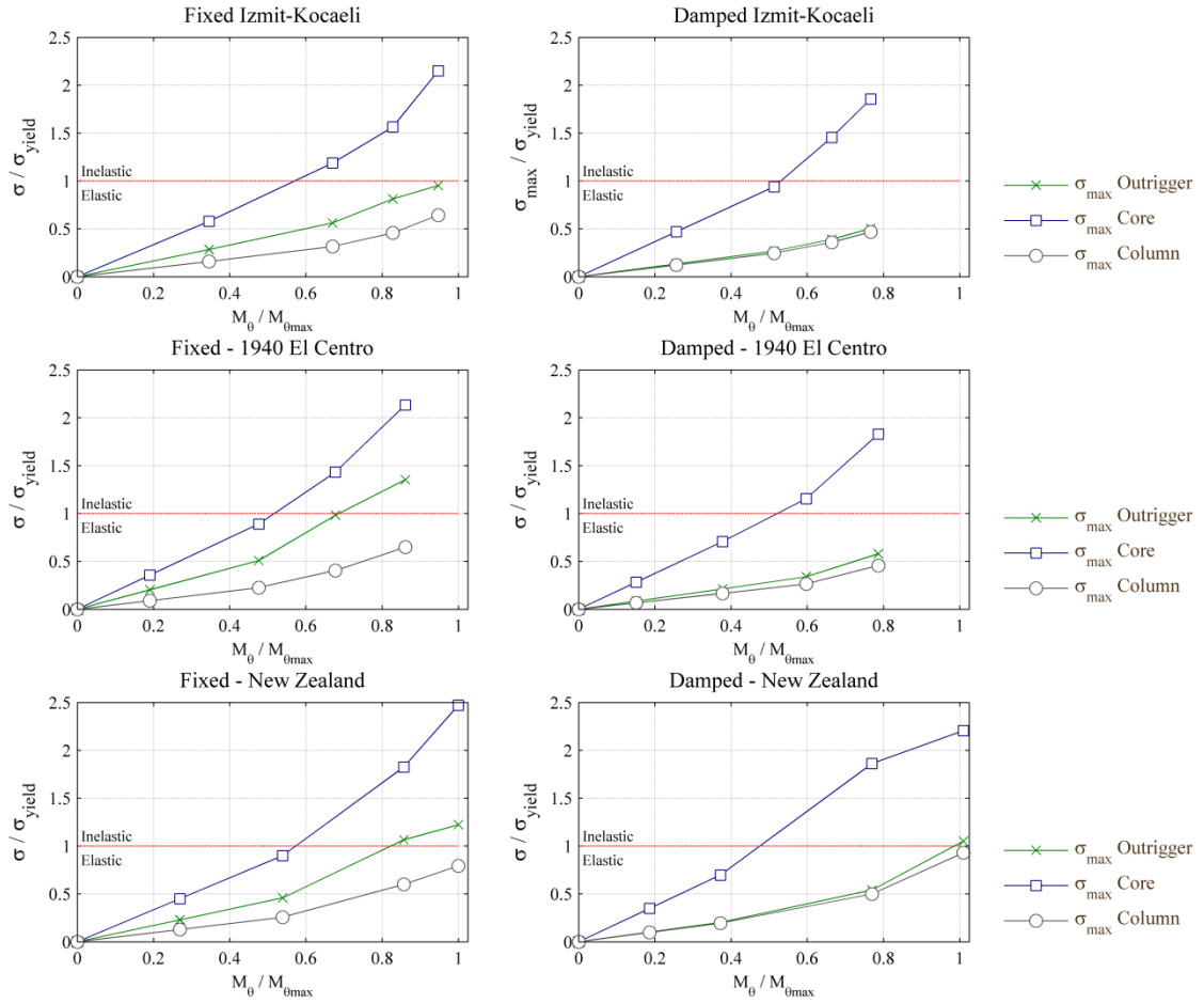
Figure 31: Normalized stress (actual/yield) to normalized overturning moment of the fixed/damped outrigger structures under different earthquake levels. \lambda=0.7 , \zeta=2.0\% and C_d=1.18E+05\text{kN-s/m} (damped outrigger).
