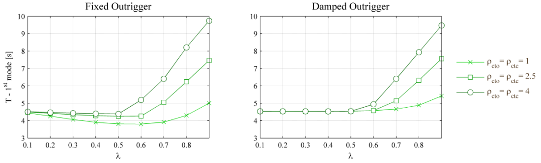
Figure 19: Influence of \lambda in the period shifts of the fixed and damped outrigger. Data points correspond to pairs \rho_{cto}-\rho_{ctc} = 1, 2.5 , and 4.
