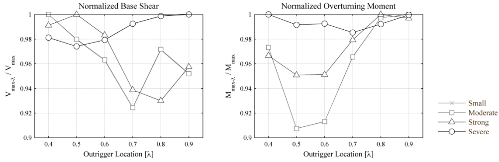
Figure 11: Normalized (actual/peak) base shear and overturning moments of the damped outrigger building ( \zeta=2\% , C_d=1.18E+08\text{kN}\cdot\text{s/m} ), subjected to four intensity levels of 1940 El Centro earthquake, with different outrigger locations ( \lambda=0.4 - 0.9 ).
