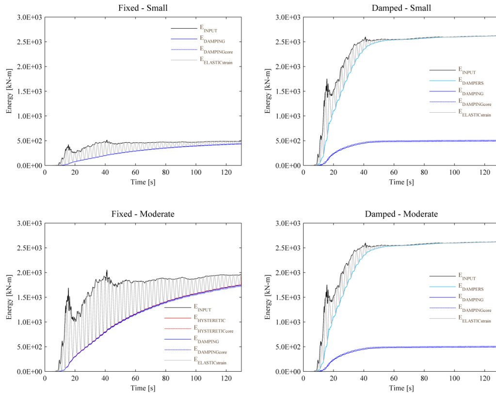
Figure 25: Energy distribution of the fixed and 1.18 \times 10^5 \text{ kN-s/m} damped outrigger structures under small and moderate levels of Izmit-Kocaeli earthquake ( \lambda=0.7 and \zeta=2.0\% ).
