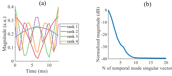
Fig. 5. (a) Modulus of the first four temporal singular vectors ( V_1(t) – V_4(t) ). (b) Normalized magnitude of the temporal mode MSV.
