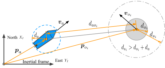
Fig. 3. Variables for collision avoidance ( d_a : size of the ASV; d_o : size of the i -th obstacle; d_{s_i} : radius of the safe region; d_{ao_i} : relative distance between the ASV and the i -th obstacle).
