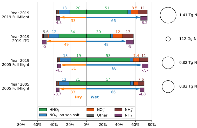
Figure 7.7: Mass of aviation-attributable nitrogen deposited globally, per species, relative to the nitrogen mass emitted by aviation as NO x , which is indicated by the quantities on the right.
