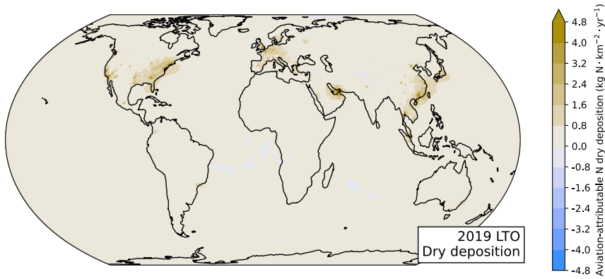
Figure D.9: Dry nitrogen deposition flux due to 2019 LTO emissions.
