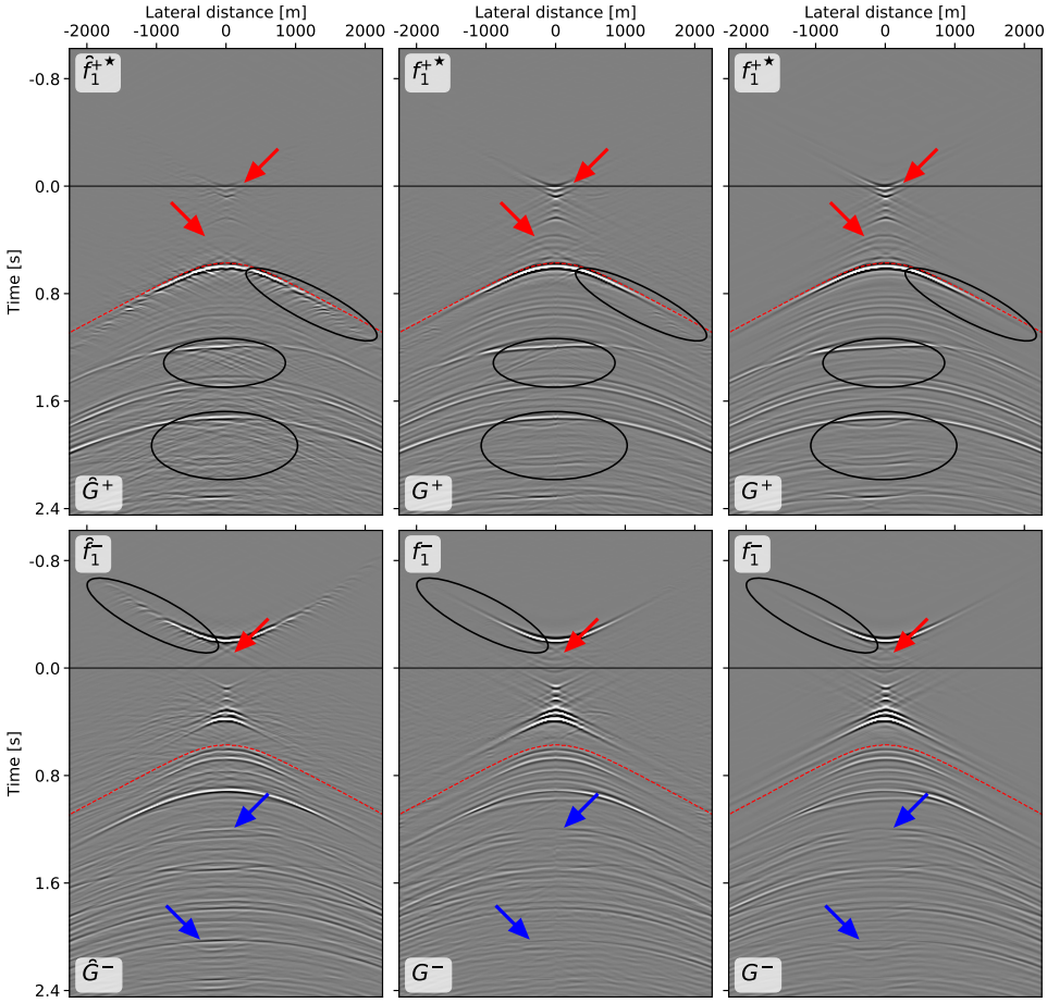
Figure 2.3: The top row shows the time-reversed downgoing focusing function ( \{\hat{f}_1^+\}^* ) and downgoing Green's function ( G^+ ), and the bottom row shows the upgoing focusing function ( \hat{f}_1^- ) and upgoing Green's function ( G^- ), the star superscript denotes time-reversal. The dashed, red lines indicate the separation between the focusing- and Green's functions. The left column shows the result of irregularly sampled data after 12 iterations of the standard Marchenko scheme. The middle column shows the results when using our scheme on the same data (Figure 2.1), again 12 iterations are used. Finally, the 3rd column shows the reference result, obtained after 12 iterations of the standard Marchenko scheme with well-sampled data. Each panel is scaled with its maximum value. The arrows and ellipses show artifacts arising from the irregular sampling. Distortions caused by the irregular sampling are indicated with the ellipses. The red arrows show events that deviate in amplitude or are missing altogether. Finally, the blue arrows mark erroneous reflectors.
