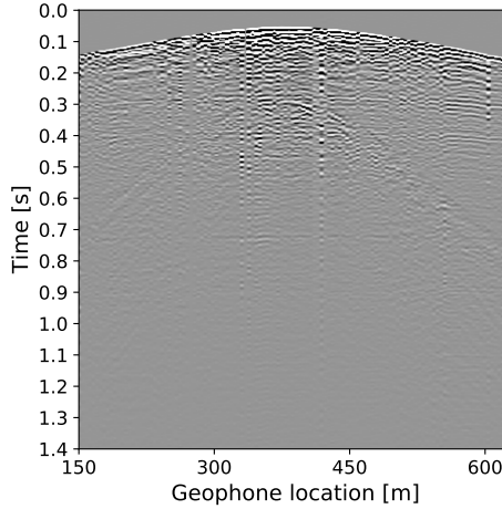
Figure A.3: Response to dynamite source at (x,z)=(375,100)\text{m} , registered by vertical-component geophones at the surface.
