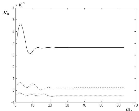
Fig. 1 The quantities \kappa_n(\omega_*) for n = 1 (solid curve) n = 2 (dashed curve) and n = 3 (dotted curve). The \omega_* ranges in the interval [0, 70] on the horizontal axis. The parameters are \alpha = 1 , \gamma = 0.1 , \phi = \pi/2 , \varepsilon_a = 0.1 , \varepsilon = 0.001 , p_0 = 1 and b_0 = 0.5
