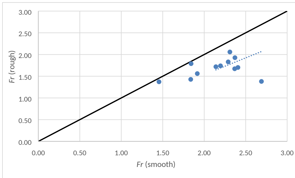
Figure 7. Comparison of Fr numbers of rough and smooth bed experimental conditions for the range of experimental conditions provided in Table 1.
