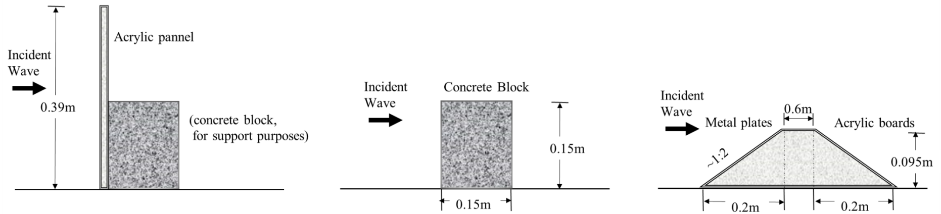
Figure 5. The structure types tested [not to scale]. From left to right, “high vertical wall”, “low vertical wall” and dyke.
