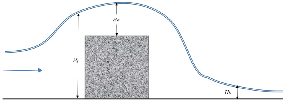
Figure 9. Wave parameters used to analyse the overtopping wave. H_f , H_o and H_b represent maximum values of the surface profile of the wave as it impacts, overtops and runs past the wall. These values were obtained from WG3, WG5 and WG6, respectively.
