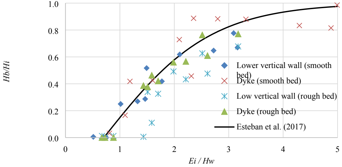
Fig.11. Relationship between the ratio of wave depth after the wall [ H_b ] to the incident wave height [ H_i ] and the E_i / H_w
