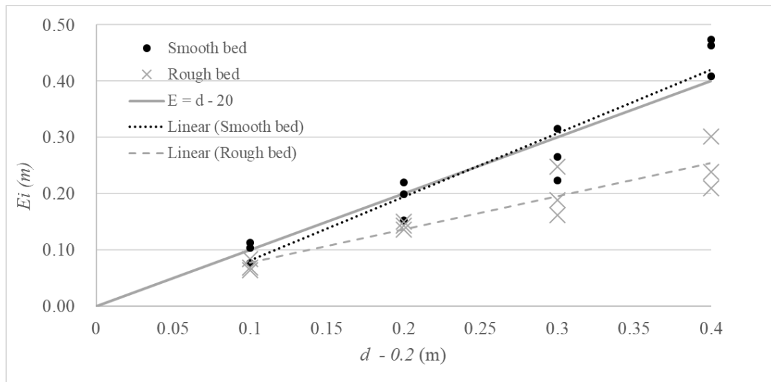
Figure 10. Relationship between E_i and static head at the edge of the gate for the high seawall
