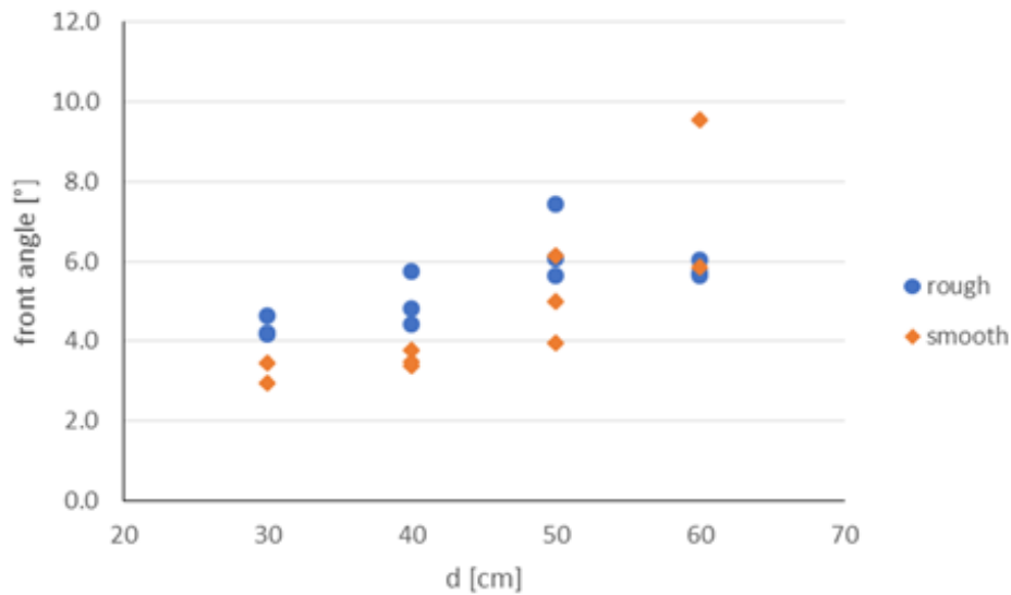
Figure 8. Comparison of direct video measurement of front slope angle for smooth and rough beds, for different water depths ( d ) in the reservoir.
