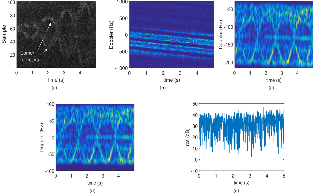
Fig. 12. (a) range-compressed and azimuth-uncompressed signal; (b) STFT of the azimuth signal; (c) STFT of the preliminary compensated and filtered azimuth signal; (d) STFT of the m-D signal; (e) the uncalibrated RCS of the target.
