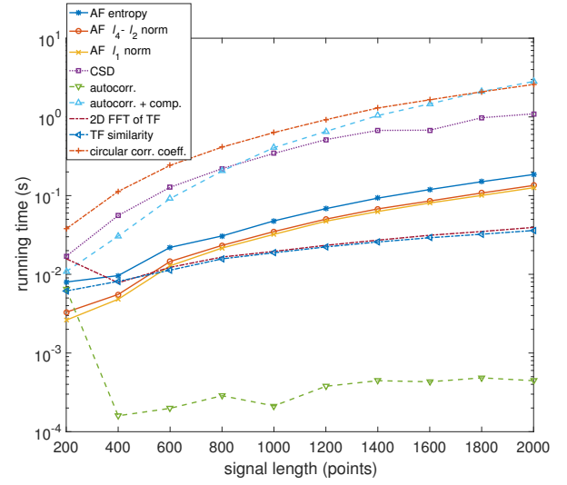
Fig. 8. Running time of the estimation methods.
