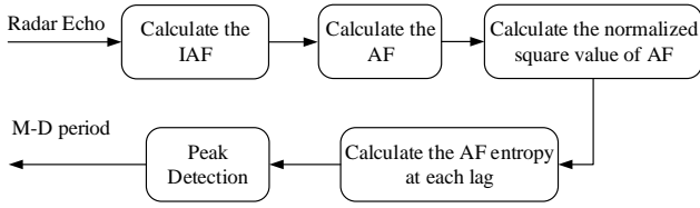
Fig. 1. Flowchart of AF entropy-based m-D period estimation.
