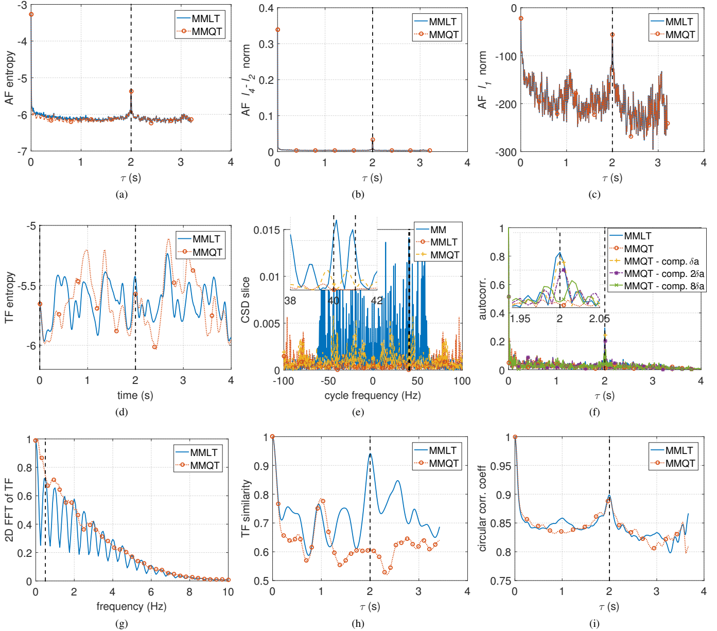
Fig. 6. Estimation Statistics. (a) AF entropy; (b) AF l_4-l_2 norm; (c) AF l_1 norm; (d) TF entropy; (e) slices of CSD; (f) autocorrelation (the dash-dot lines with circle, square and asterisk markers denote the results by integrating translation compensation with different search intervals); (g) 2D FFT of TF; (h) TF similarity; (i) circular correlation coefficients. The true m-D period/frequency is indicated by a black dashed vertical line in (a), (b), (c), (e), (f), (g), (h), (i). While in (d) and (e), two vertical lines with distance of the true m-D period and two multiples of the m-D frequency are plotted which means that the statistics should have periodic peaks or periodic pattern at these two instants if they are effective.
