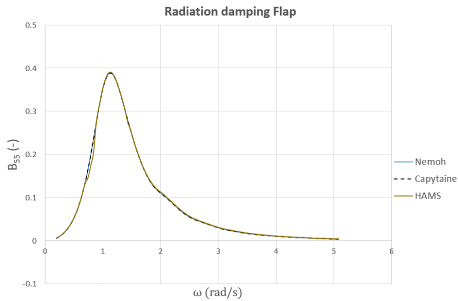
Figure 11. Pitch radiation damping for OSWEC
