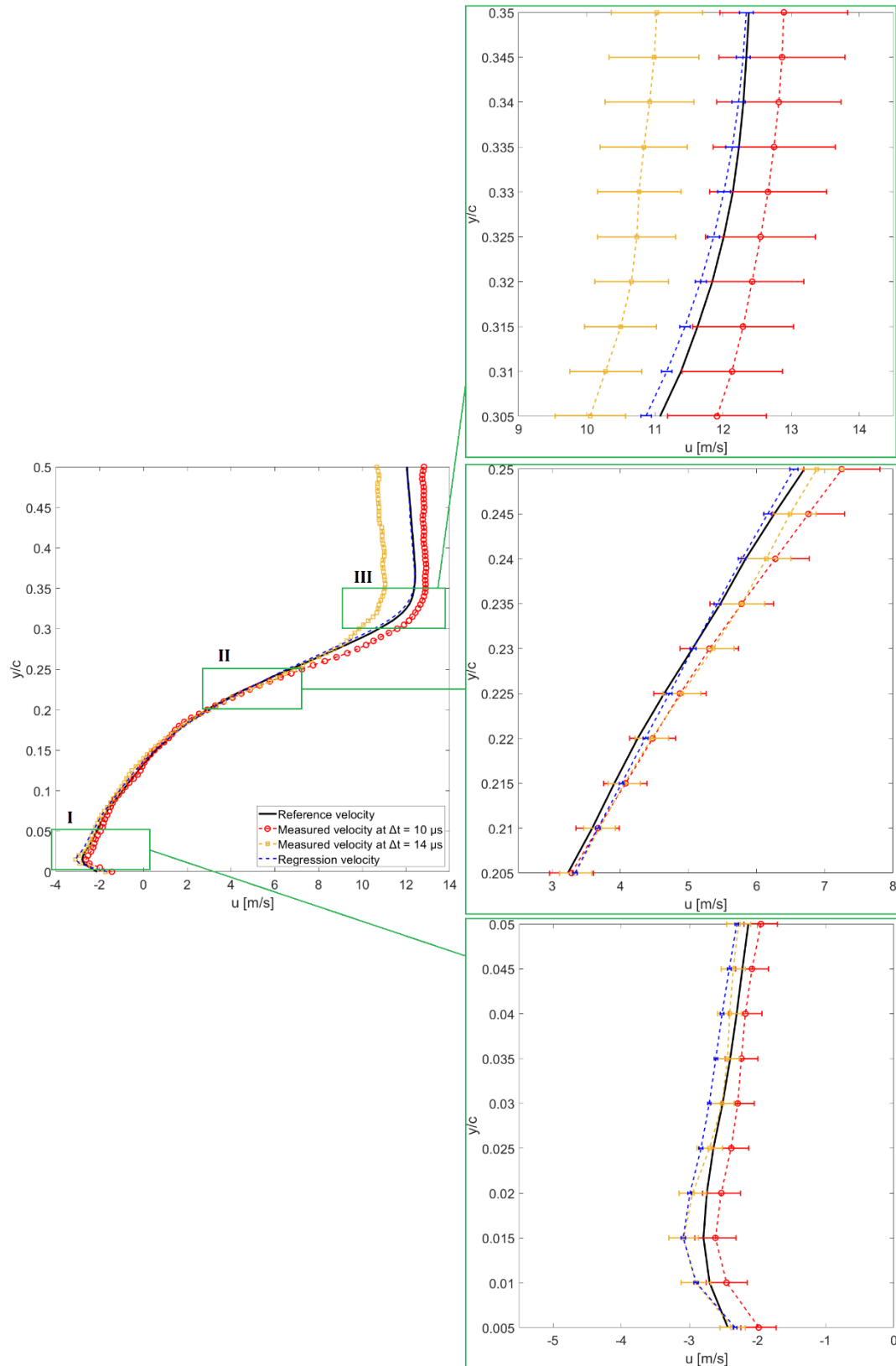
Figure 7: Plots of reference velocities, measured velocities at \Delta t equal to 10 \mu s and 14 \mu s , and regression velocities with uncertainty bands in the wake flow experiment [The velocities are plotted at x/c = 0.85 , where y/c = 0 at the surface of the wing and increases in the downward direction away from the surface as shown by a vertical dotted line in Fig. 3(b) and Fig. 6]
