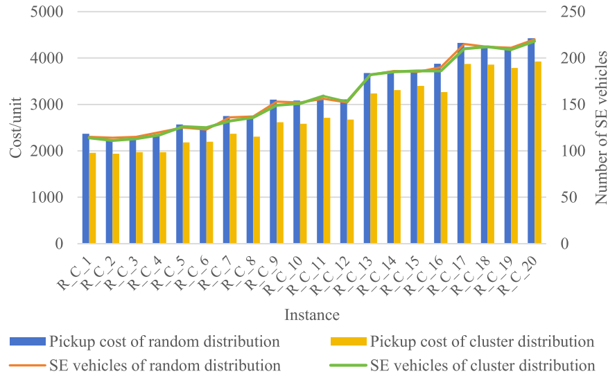
Fig. 12. Comparison of pickup cost and SE vehicles between the two distributions.
