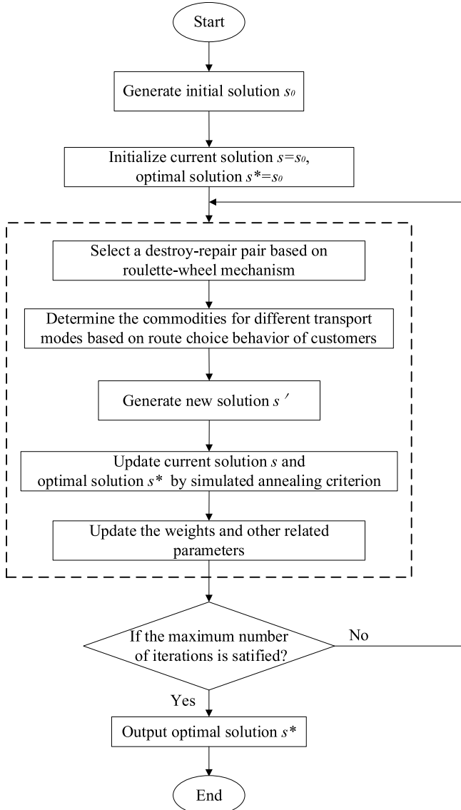
Fig. 6. Flowchart of the ALNS algorithm.
