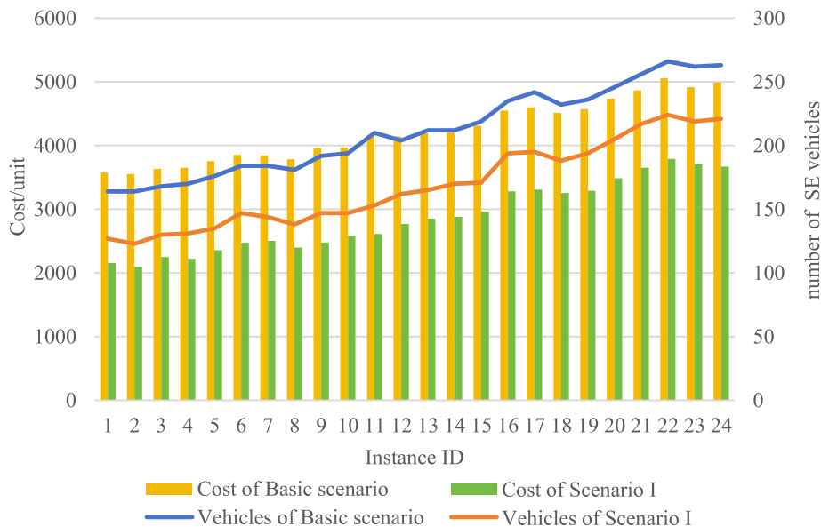
Fig. 8. Cost and vehicles in the delivery stage between the Basic scenario and Scenario I.
