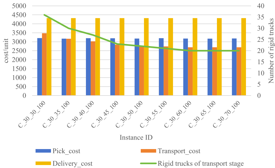
Fig. 14. Impact of rigid truck capacity.
