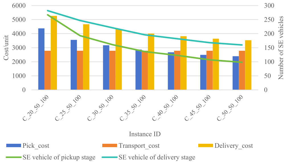
Fig. 13. Impact of SE vehicle capacity.
