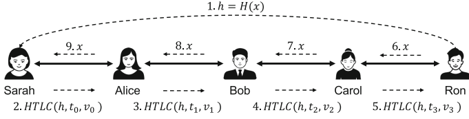
Fig. 1. A multi-hop payment with HTLCs. h denotes \text{MHP}[i].\text{cond} where x is the corresponding preimage, and t_i and v_i represents \text{MHP}[i].TL and \text{MHP}[i].\text{amt} .
