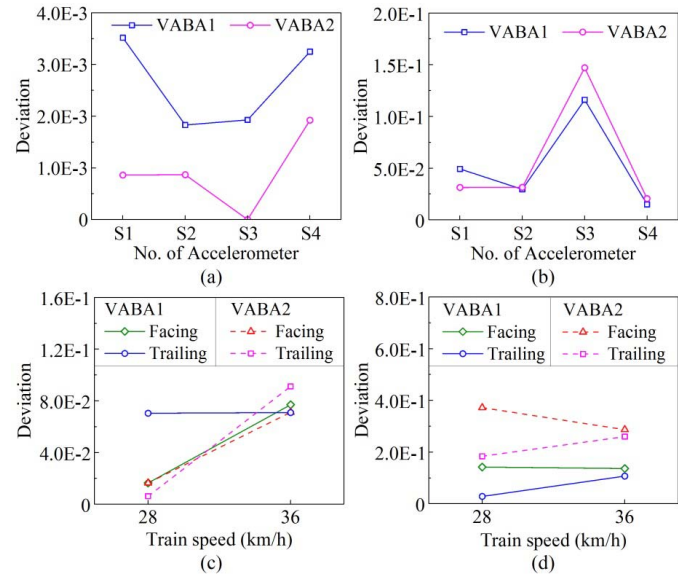
Fig. 17. Uncertainty of (a) and (b) hammer test and (c) and (d) ABA measurement evaluated by standard deviation among tests. (a) Crossing natural frequencies at VABA1 and VABA2. (b) Accelerance at crossing natural frequencies. (c) Major ABA frequencies VABA1 and VABA2. (d) GWPS at major ABA frequencies.
