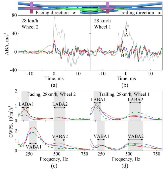
Fig. 11. Comparison between the LABA and the VABA. The signals were acquired from the rear wheel at 28 km/h. (a) and (b) Time history. The solid line (—), dashed line (---), and dotted line (···) indicate the LABA from three independent tests, while the shadow solid line (—) indicates the VABA. (c) and (d) GWPS of the ABA. Letters VABA1 and VABA2 indicate the major frequency bands of the VABA, while letters LABA1 and LABA2 indicate the major frequency bands of the LABA.
