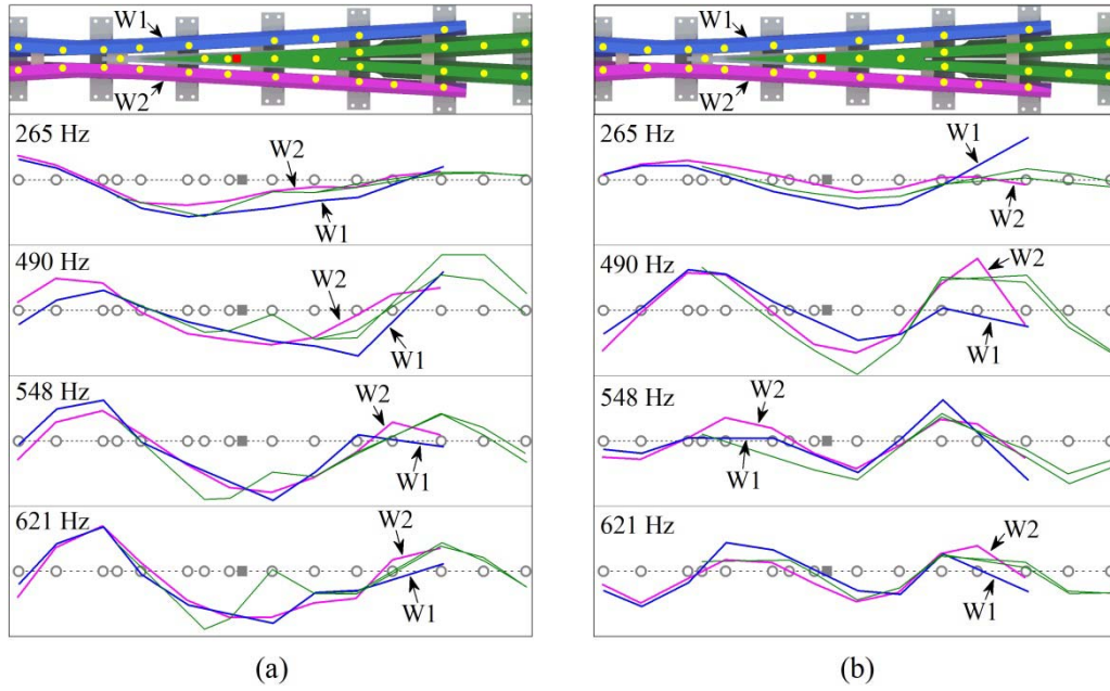
Fig. 15. ODSs of crossing rails at the crossing natural frequencies of 265, 490, 548, and 621 Hz. (a) Phase with the maximum impact force. (b) Phase where the impact force reached zero. The symbols (■) and (○) indicate the impact position and the sensor position. Letters W1 and W2 indicate the nonsynchronized vibrations of the two wing rails.
