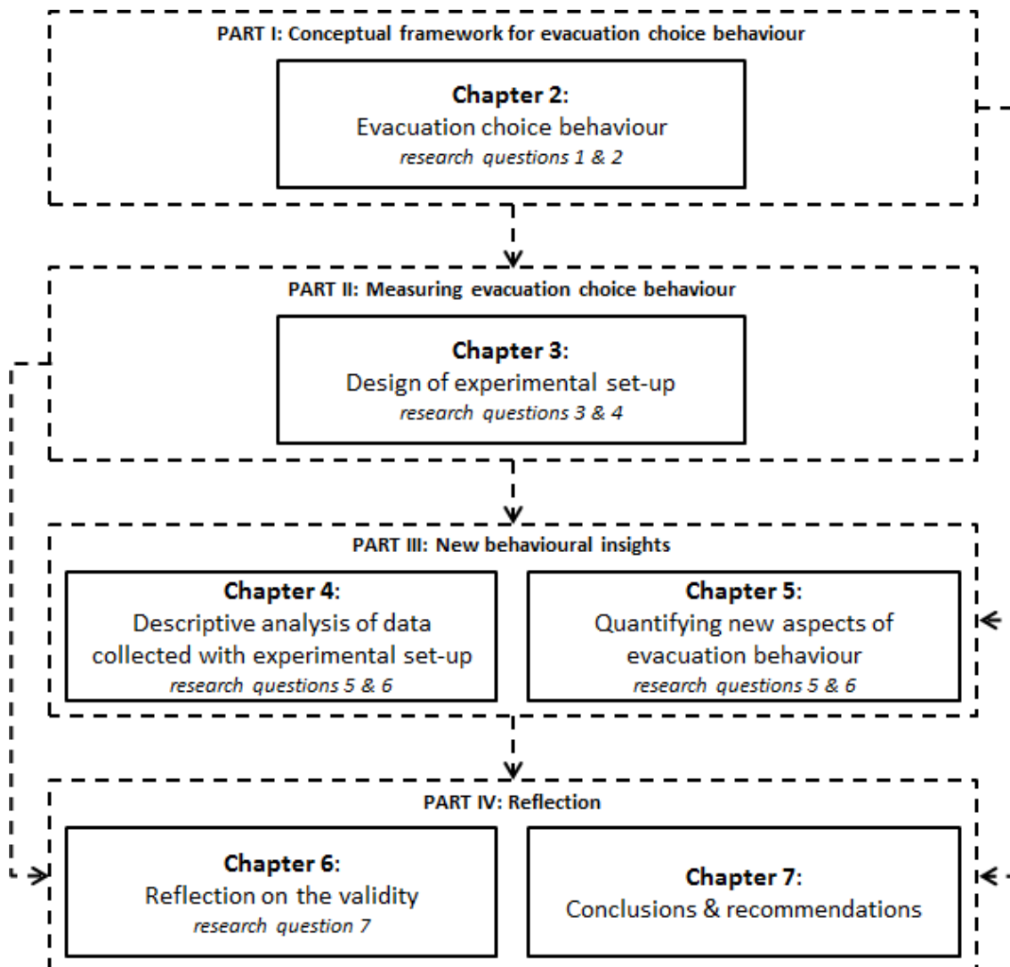
Figure 1.3: Thesis outline
