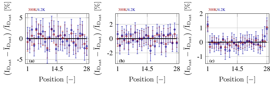
FIGURE 12. Relative I_{Dsat} ( I_D|V_{DS}=V_{GS}=1.1 V) values as a function of device position for NMOS devices at RT (red) and LHT (blue): a) W/L = 120n/40n ; b) W/L = 360n/120n and c) W/L = 1.2\mu/400n . Zero deviation emphasized by the black lines and error bars indicate 95% confidence intervals.
