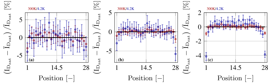
FIGURE 13. Relative I_{Dsat} ( I_D|V_{DS}=V_{GS}=1.1 V) values as a function of device position for PMOS devices at RT (red) and LHT (blue): a) W/L = 120n/40n ; b) W/L = 360n/120n and c) W/L = 1.2\mu/400n . Zero deviation emphasized by the black lines and error bars indicate 95% confidence intervals.
