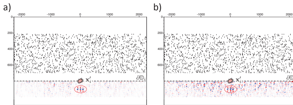
Figure 5 (a) Result of Marchenko imaging, applied to the target zone. (b) Result of standard imaging.
