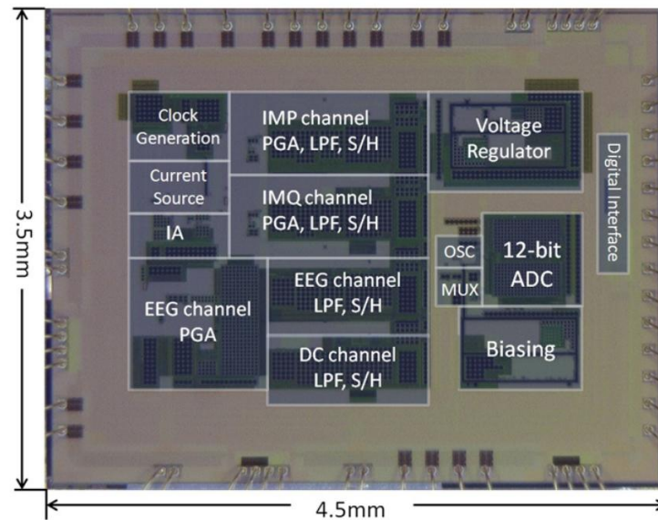
Fig. 13. Chip photograph
