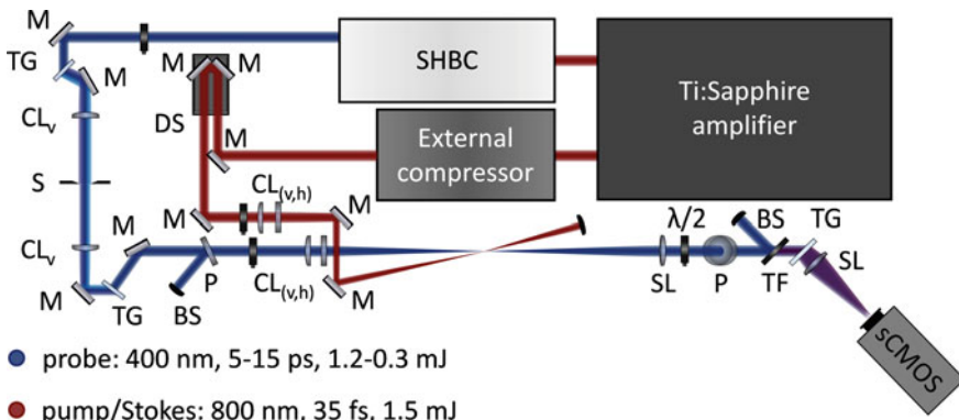
Fig. 13.5 Schematic drawing of the two-beam fs/ps 1D-CARS imaging instrument developed in [47]. A single Ti:sapphire ultrafast regenerative amplifier system is employed to generate the 35 fs pump/Stokes and the \sim 5 –15 ps probe pulses. Cylindrical lenses, mounted in an astigmatic focusing configuration, form the laser beams into two sheets at the measurement location, where they cross to form a \sim 1.3 mm measurement line. TG, transmission grating; S, slit; CL, cylindrical lens with vertical (v) and horizontal (h) symmetry axes; \lambda/2 , half-wave plate; B, burner; P, polarizer; SL, spherical lens; M, mirror
