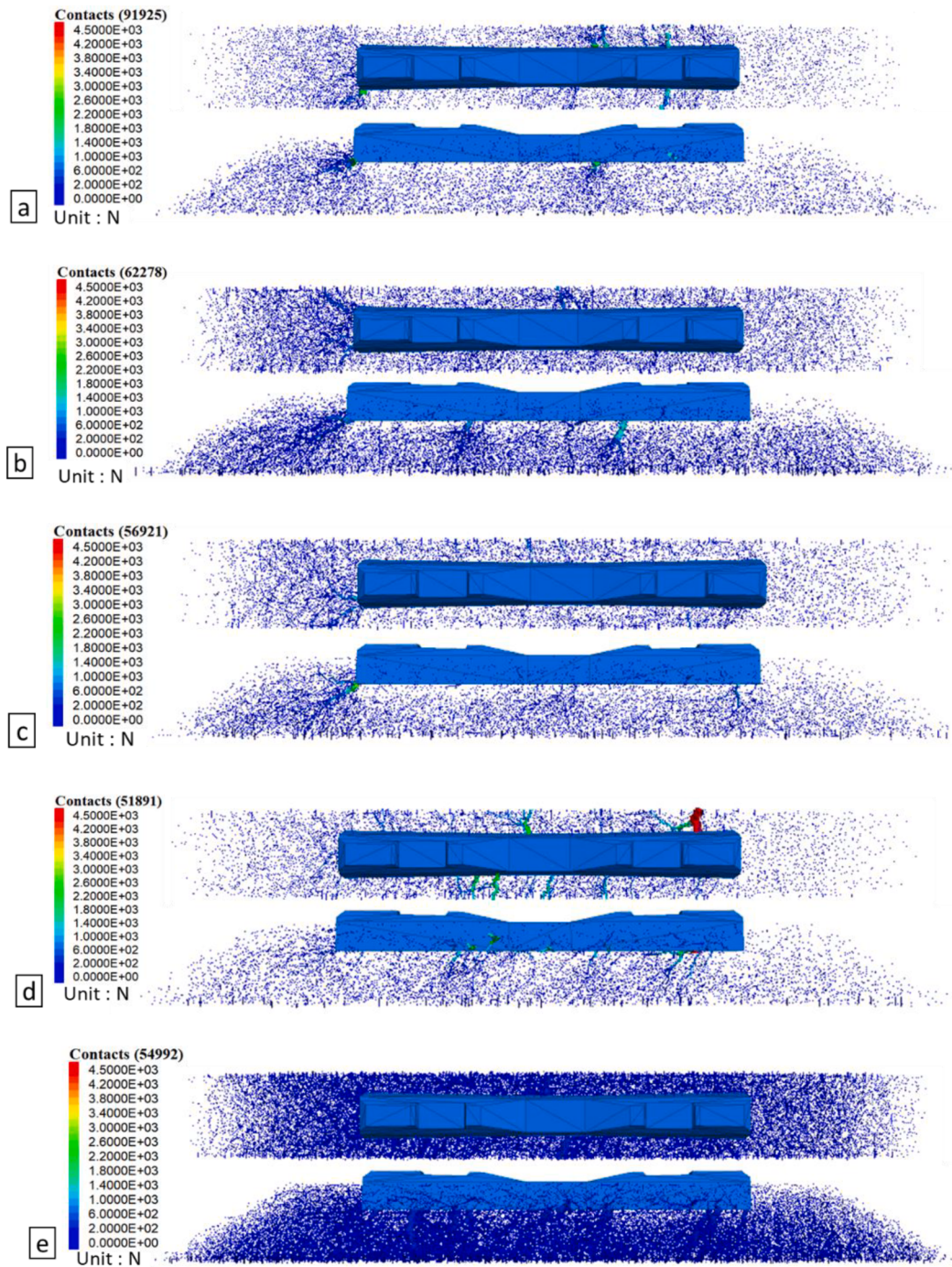
Fig. 20. Contact force chain after 5 mm sleeper displacement: a) Reference model (all particles are clump), b) Multi-layer model (Half clump and half ball, by height), c) Optimised multi-layer model (based on most influential ballast area), d) Ball-built model (with rolling resistance), e) Ball-built model (without rolling resistance).
