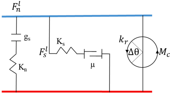
Fig. 9. Linear contact with rolling resistance.
