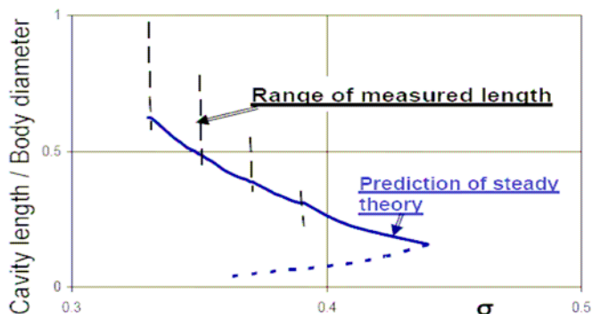
Figure 3: Comparison of observed (by Ceccio and Brennen, [9]) and computed (by Amromin, [6]) cavity lengths on the ITTC axisymmetric body (0.05m diameter).
