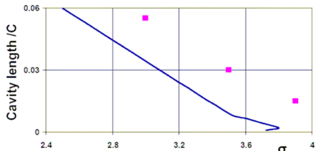
Figure 4: Comparison of computed and observed (after Amromin et al, [10]) cavity length on NACA-16009 hydrofoil with C=0.1m at 5 degree angle of attack in a narrow water tunnel.
