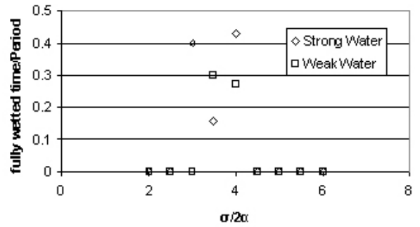
Figure 7. Fully wetted time on a stainless steel Cav 2003 hydrofoil at 4° angle of attack
