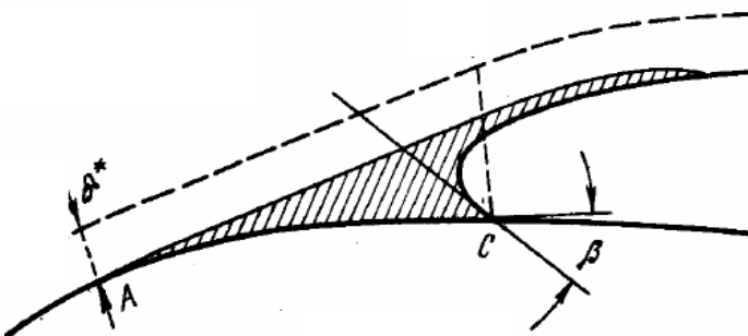
Figure 1: Sketch of cavity detachment zone. Striped area is the zone of laminar separation caused by the cavity: \delta^* is thickness displacement of the laminar boundary layer that separates from the wall and reattaches to the cavity surface. Adapted from Arakeri [5].
