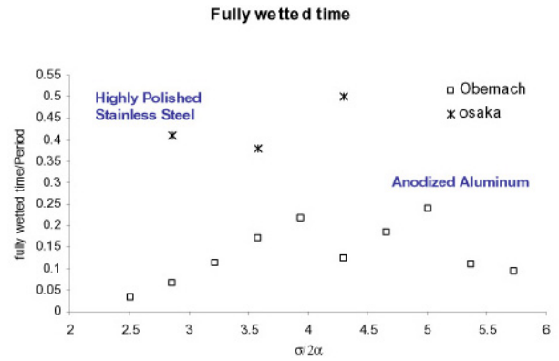
Figure 6. Fully wetted time on a NACA 0015 hydrofoil (Kawakami et al, 2008)
