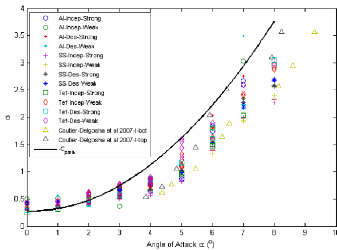
Figure 10 Inception Data for the Cav 2003 hydrofoil
