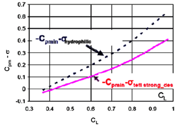
Figure 11 Calculation of -C_{pm} - \sigma by Amromin [6]
