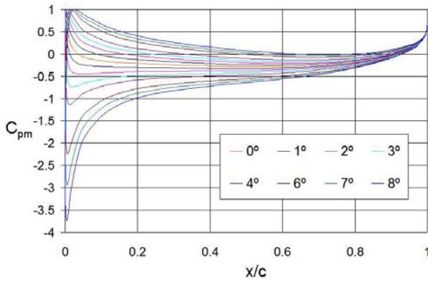
Figure 9. Pressure coefficient, Cav 2003
