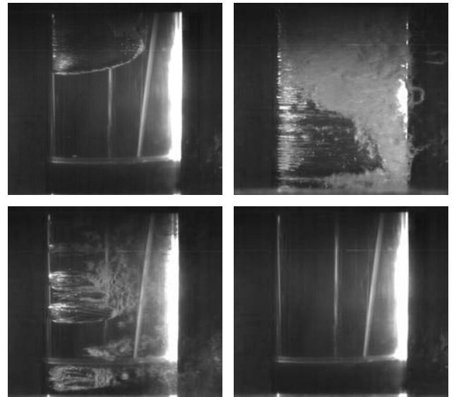
Figure 8. Stainless steel in weak water. \alpha = 4^\circ , \sigma/2\alpha = 4 . View of cavitation at different stages in the oscillation cycle: Top Left: t = 0.142 period Top Right: t = 0.585 period Lower Left: t = 0.803 period Lower Right: Fully Wetted One period was equivalent to a time of 0.06 seconds. Flow is from left to right
