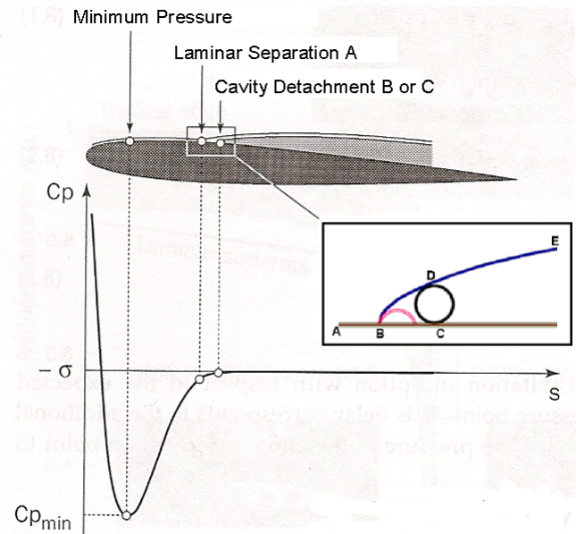
Figure 2: Illustration of the viscous-inviscid iteration concept. As shown, the pressure distribution upstream of the cavity corresponds to pressure less than vapor pressure (tension). A is the point of laminar boundary layer separation from the surface 1 . The inset illustrates the comparison of the cavity detachment regions for hydrophilic and hydrophobic surfaces. The cavity boundary is the curve BDE for a Teflon surface with a contact angle \beta = \pi/2 and the curve CDE for an aluminum surface with an assumed contact angle \beta=0 . (Adapted from Franc and Michel, [4]).
