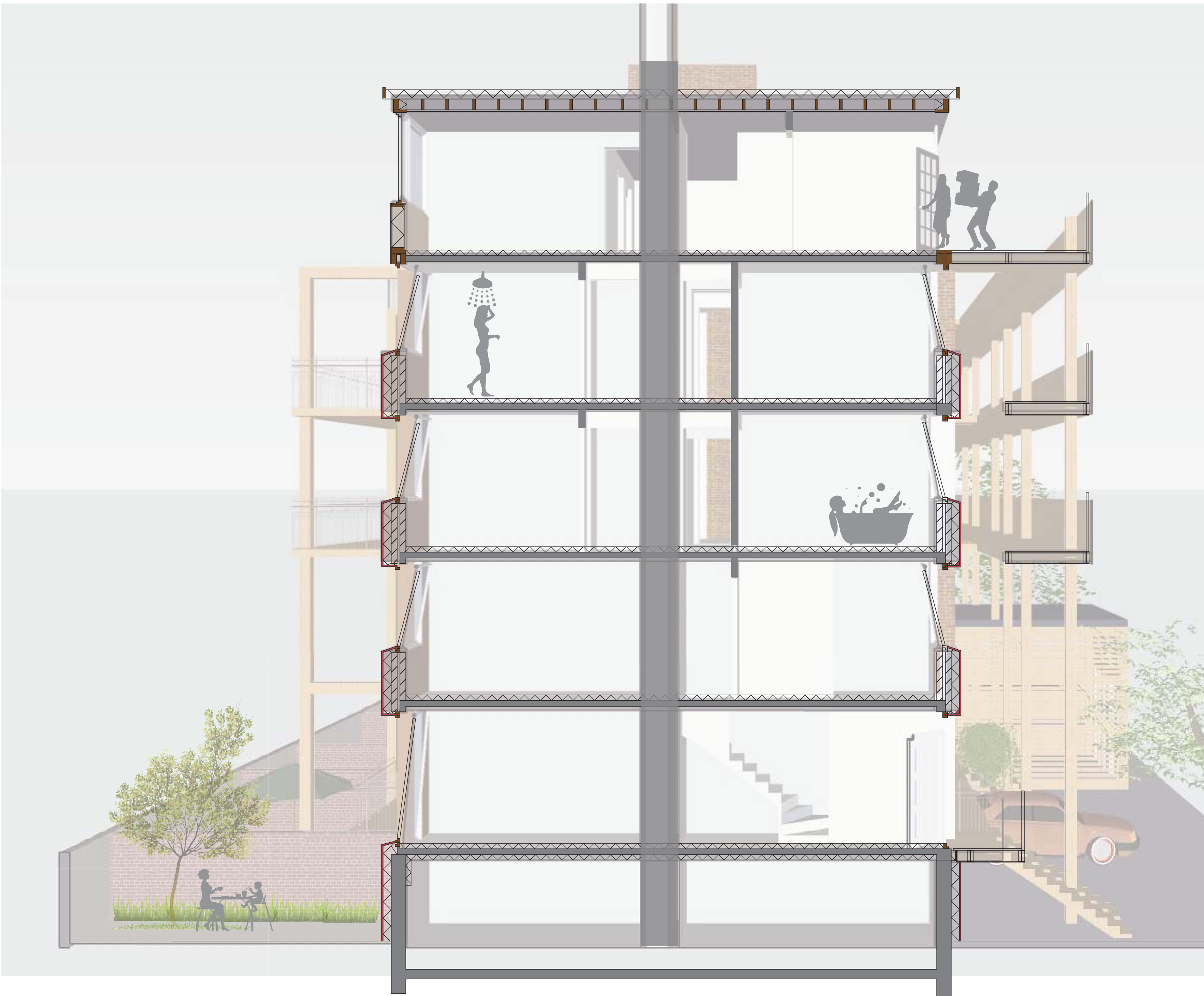
Section BB`
