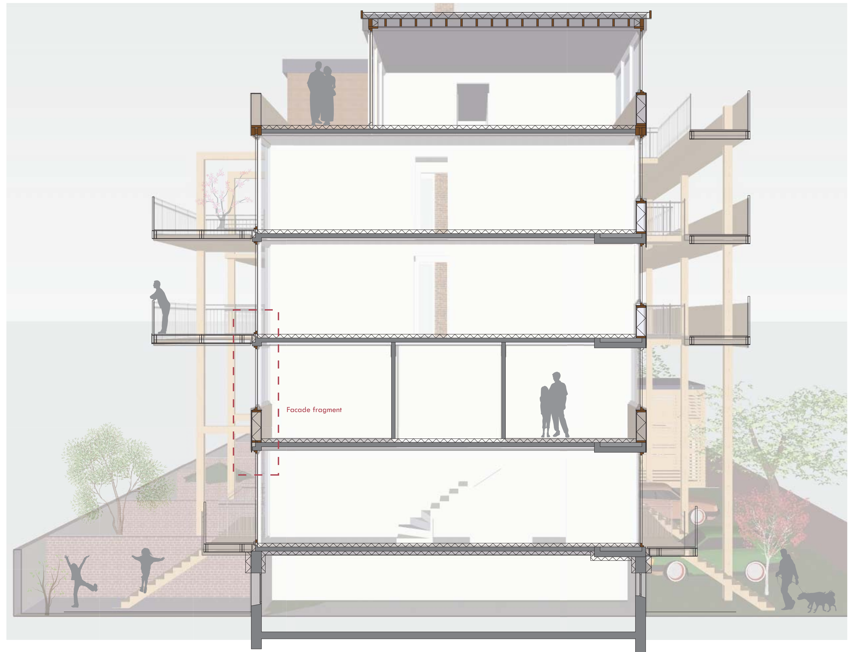
Section AA`
