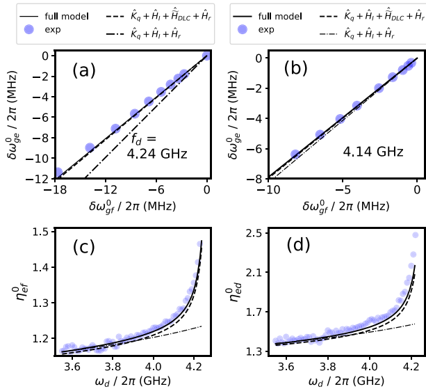
Fig. 2 | Identifying drive-induced longitudinal coupling (DLC) from multi-level spectroscopy. We investigate drive frequency \omega_d near \omega_r^0 . Circles denote experimental data. Lines indicate theoretical calculation based on the corresponding Hamiltonian models in legend. a, b We plot the frequency shifts in ge transition ( \delta\omega_{ge}^0 ) with respect to that of gf transition ( \delta\omega_{gf}^0 ) for \omega_d/2\pi = f_d = 4.24 GHz and \omega_d/2\pi = f_d = 4.14 GHz, respectively. c, d We plot dimensionless quantities \eta_{ef}^0 = \frac{1}{2} \delta\omega_{gf}^0 / \delta\omega_{ge}^0 |_{\Omega_d \rightarrow 0} and \eta_{ed}^0 = \frac{1}{2} \delta\omega_{gd}^0 / \delta\omega_{ge}^0 |_{\Omega_d \rightarrow 0} , while sweeping \omega_d . Errors are less than the size of symbols, and thus not presented in the plots. The errors are statistical and originated when extracting \delta\omega^0 from data.
