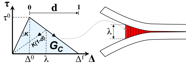
Fig. 1 Constitutive response for traction-separation cohesive elements.
