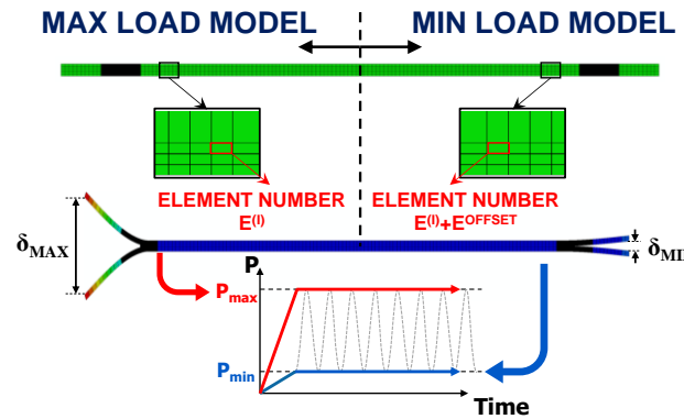
Fig. 3 FE application of Min-Max Load Approach.
