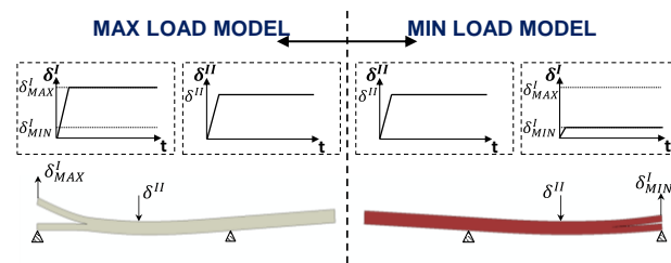
Fig. 13 Min-Max Load Approach for modified MMB specimen.
