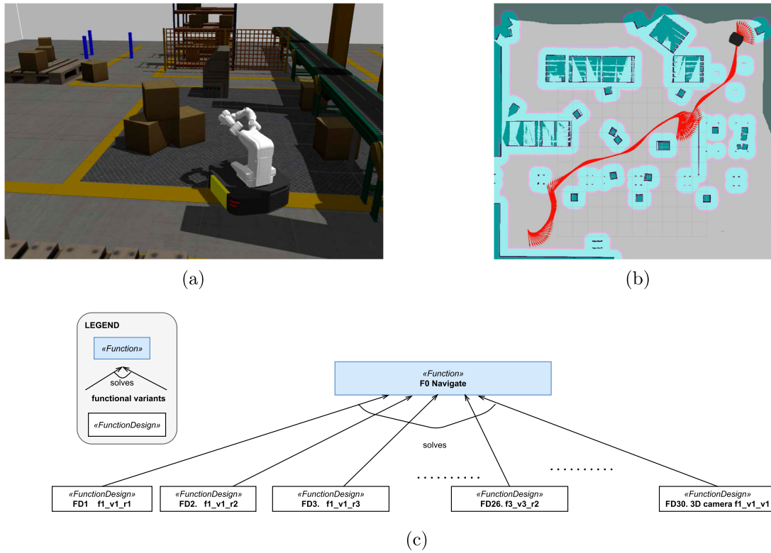
Figure 6. Mobile Manipulator in a factory. (a) Simulation of the mobile manipulator in a factory. (b) An example route of the mobile manipulator navigating. (c) TOMASys model of the control architecture of the mobile manipulator navigating.
