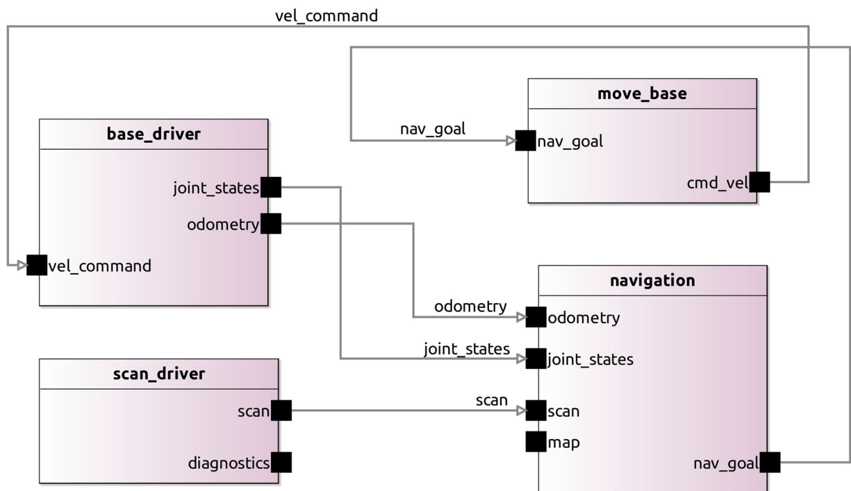
Figure 3. Example RosSystem model for the system in Figure 2.
