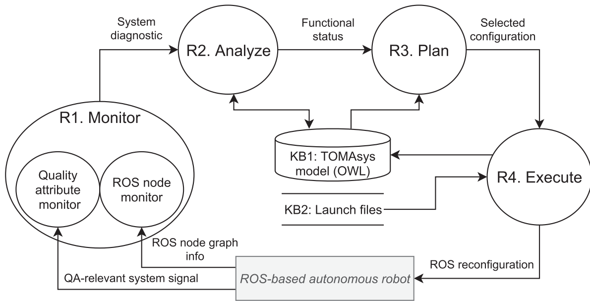
Figure 4. Data flow diagram for the runtime operation of the MAPE-K loop implemented by the MROS Meta-controller.
