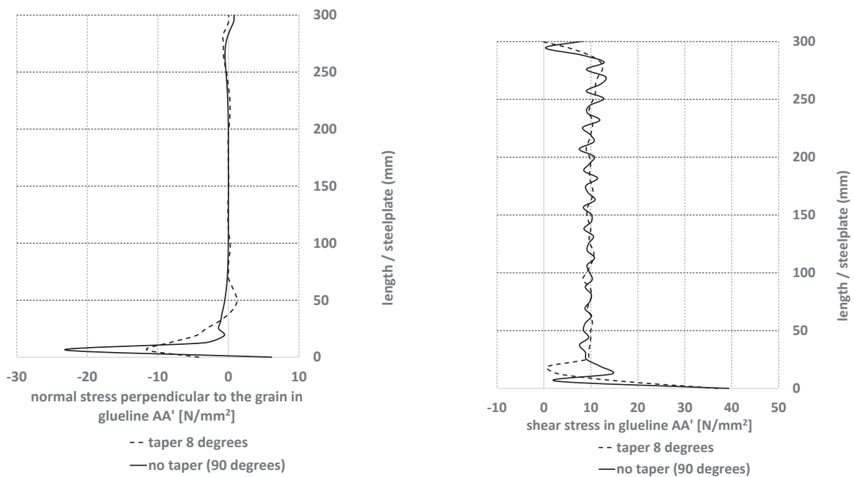
Figure 7: Shear stress in the glueline AA' for hardwood
