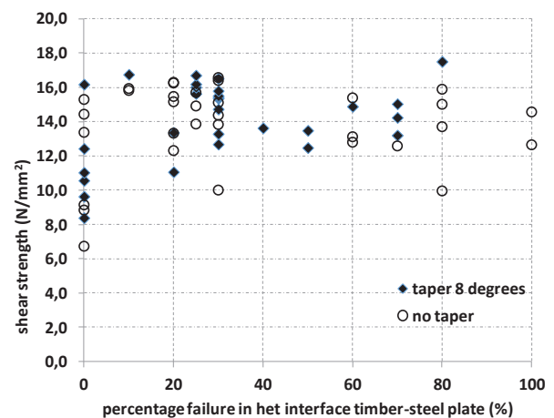
Figure 13: Shear test results for massaranduba plotted against percentage failure in the interface divided in to specimens with and without tapered steel plates.
