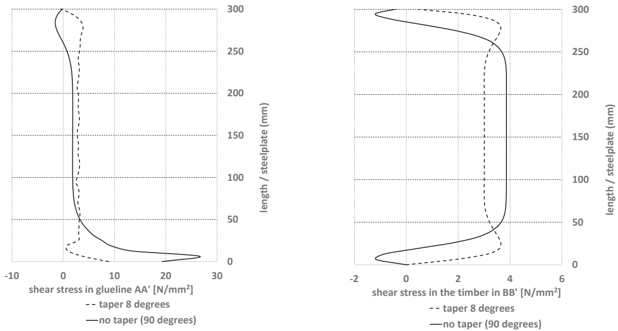
Figure 4: Shear stress in the glueline AA' for softwood.
