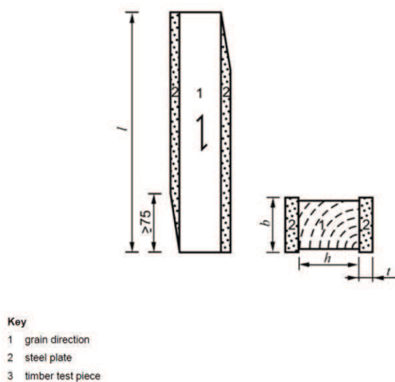
Figure 1: Timber test piece with glued on steel plates according to EN 408.
